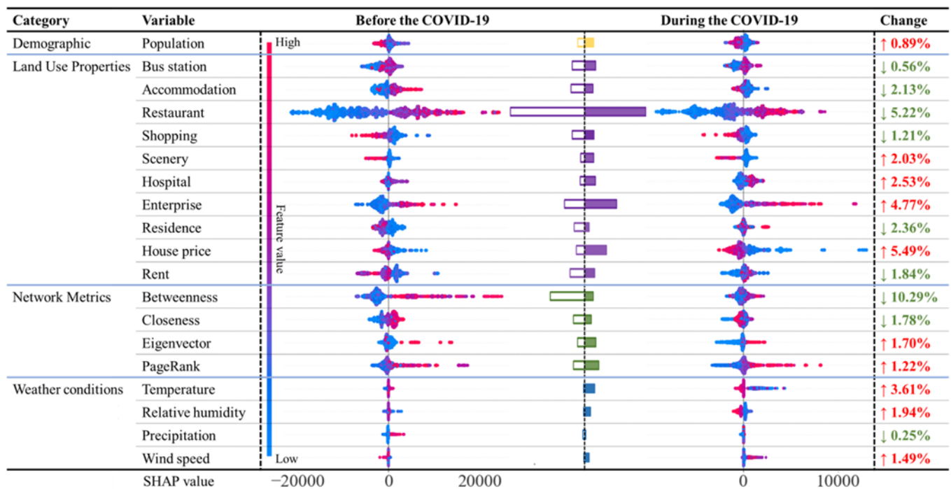
Figure 4 The SHAP summaries plot of all variables and the relative feature importance. The plot conveyed the impact of each sample's attributes on subway ridership, with the colors denoting the magnitude of the feature value and position reflecting the scale of the SHAP value (Positive and negative SHAP values denote affirmative and adverse contributions to subway ridership, respectively). The histograms visually delineated the shifting relative importance of each variable's impact on subway ridership, distinguishing between the pre-COVID-19 and COVID-19 periods. The "Change" indicated how much the relative importance had changed before and during the COVID-19.
