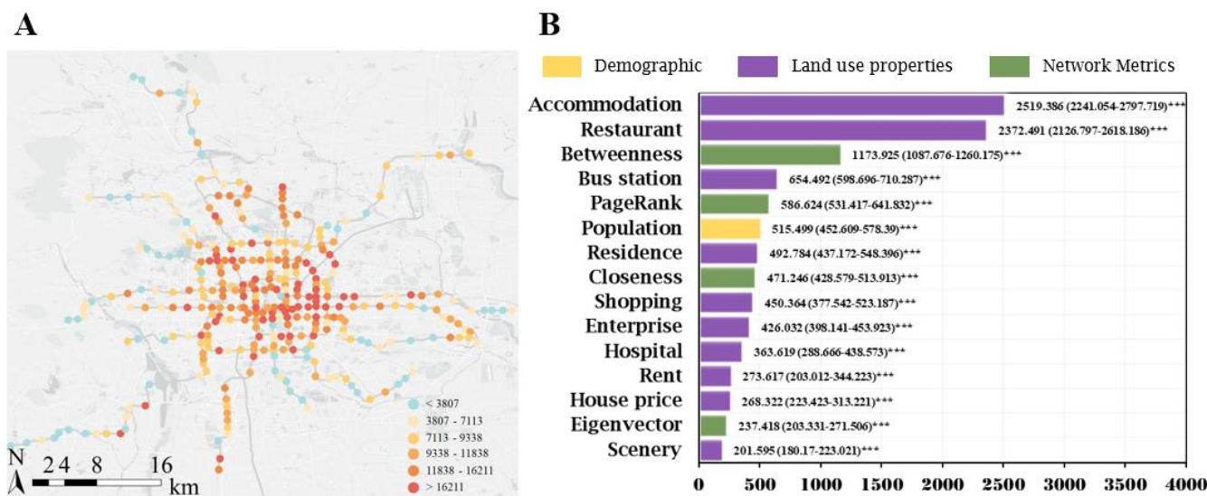
Figure 3 The causal estimates of COVID-19 on subway ridership and their influencing factors. (A) The spatial distribution of causal estimation under X-Learner, indicates the reduction in tap-in ridership as a result of the intervention of COVID-19. (B) Permutation importance scores and Confidence Interval (95% CI). *** means p < 0.001 (a p-value of 0.01 indicates that there is a 1% chance that the feature is useless or harmful and a 99% chance that the feature is useful).
