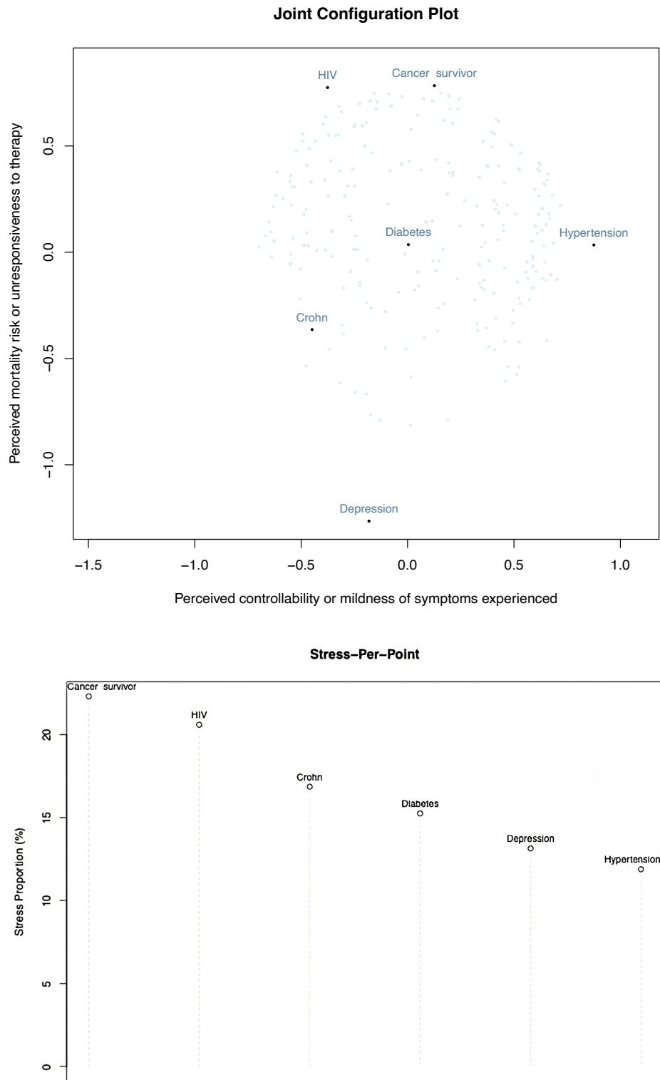
Figure 1. Top: Two-dimensional unfolding solution plot of individuals (light dots) and objects (dark dots). Bottom: Stress Per Point diagram illustrating the contribution of each object to the overall stress of the solution.
