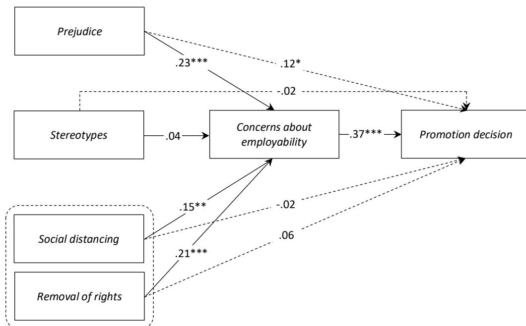
Figure 2. Structural equation model with prejudice, stereotypes, and discriminatory attitudes (i.e., social distancing and removal of rights) as exogenous variables, concerns about employability as mediator, and
