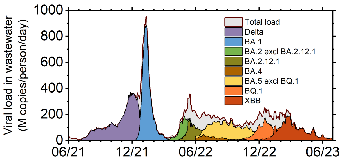
Figure 3. The 7-day simple moving average of the load of individual variants in Metro Plant influent is shown in consolidated colored bars with black outline, vs time, from June 1, 2021, to June 30, 2023. The 7-day simple moving average of the total daily SARS-CoV-2 load in Metro Plant influent is shown in consolidated gray bars with red/black outline, vs. time.
