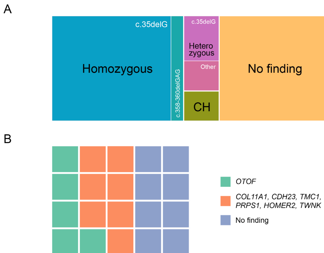
Fig 1. The distribution of patients depending on the presence of variants in different genes. A Investigated groups include conventional sensorineural hearing loss and B auditory neuropathy spectrum disorders. Abbreviations: CH – compound heterozygote.
