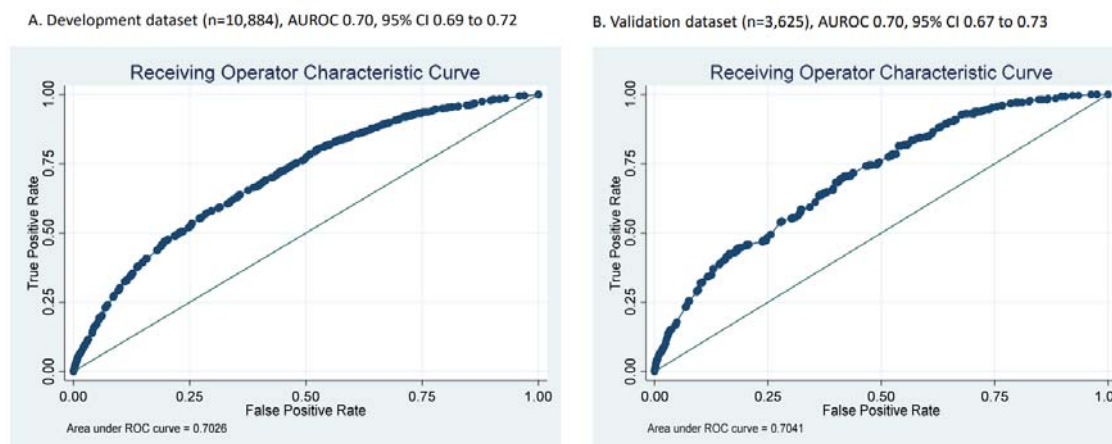
Figure 2. Receiver operating characteristic curve for the PREPARE hypoxemia clinical prediction model for children 2–59 months of age with pneumonia
