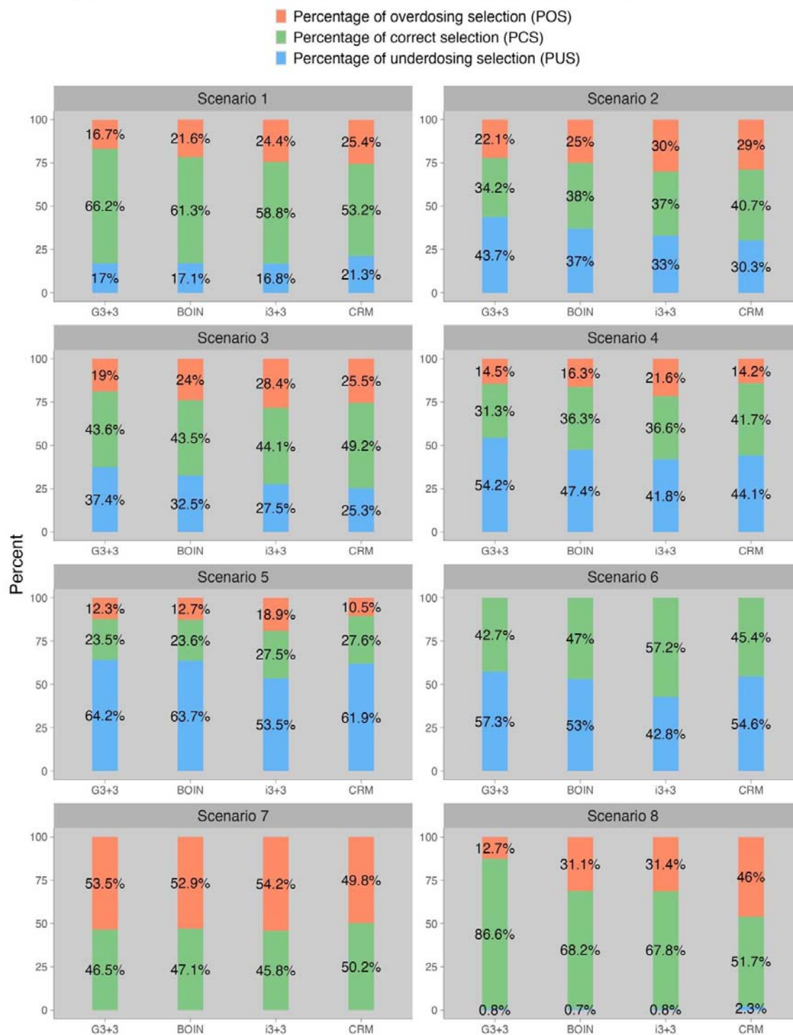
Figure 2 Operating characteristics in terms of MTD selection for the G3+3, BOIN, i3+3 and CRM designs.
