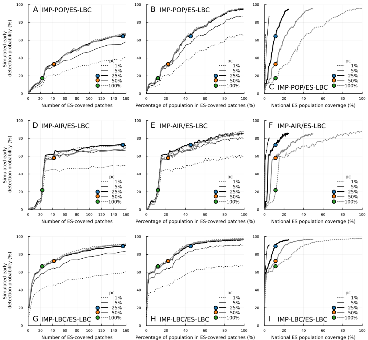
Fig S15. Sensitivity analysis of the patch-level ES population coverage, p_c , for the ES-LBC scenarios. (A, B, C) For the IMP-POP/ES-LBC scenario. (D, E, F) For the IMP-AIR/ES-LBC scenario. (G, H, I) For the IMP-LBC/ES-LBC scenario. Simulated early detection probability is plotted (A, D, G) against the number of ES-covered patches, (B, E, H) against the percentage of the population in ES-covered patches, and (C, F, I) against the national ES population coverage. The data points represent simulations where the national ES population coverage of the simulated ES layout aligns with the current coverage in South Africa (11.3%), under p_c of 25% (blue), 50% (orange) and 100% (orange). The national ES population coverage is given by the product of p_c and the percentage of the population in ES-coverage patches. It is noted that the maximum number of ES-covered patches is 1502 and the x-axis for (A, D, G) is limited to a maximum value of 160.
