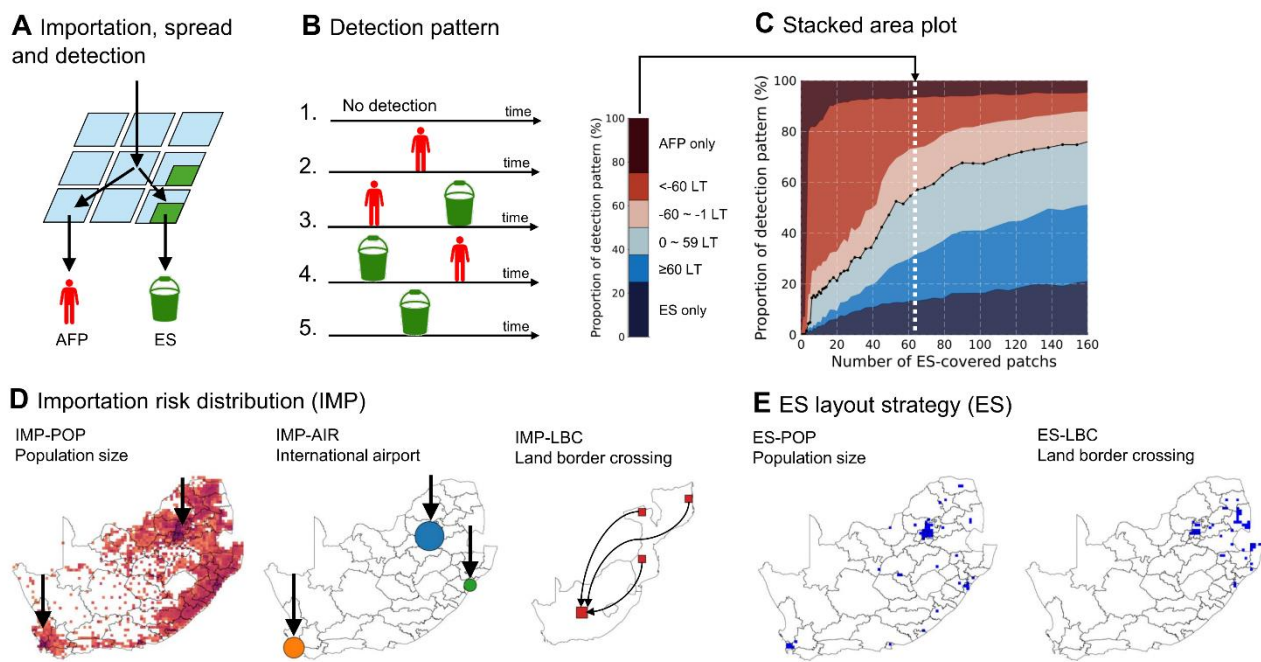
139 Fig 1. Schematic illustration of study settings. (A) Simulated importation of wild poliovirus 140 serotype 1 to South Africa, spread described by the meta-population model, and detection through 141 acute flaccid surveillance (AFP) and environmental surveillance (ES). AFP surveillance is carried 142 out across all patches whereas ES operations are confined to selected patches (in green). A patch- 143 level ES population coverage is assumed to be 25%. (B) Five detection patterns: i) No detection, ii) 144 AFP only detection, iii) earlier detection through AFP surveillance than ES, iv) earlier detection 145 through ES than AFP surveillance v) ES only detection. Detection patterns of iii) and iv) are further 146 classified based on the lead time (LT) of the first detection through ES over AFP surveillance. (C) 147 Stacked area plot of the proportion of each detection pattern against the number of ES-covered 148 patches. (D) Three importation risk distributions: i) IMP-POP corresponds to the 'Population size'- 149 based importation risk distribution and assumes importation risk is proportional to the population 150 size of each patch (indicated by orange-red colouration); ii) IMP-AIR corresponds to the 151 'International airport'-based importation risk distribution and assumes an importation risk is shaped 152 by international inbound travel volume in 2019 and approximated movement from airports. Each 153 circle denotes the international airport with a size proportional to the international inbound travel 154 volume: Blue, O.R. Tambo International Airport; Orange, Cape Town International Airport; Green,
