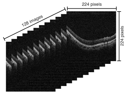
Figure 1. Schematic representation of the segmentation-free 3D convolutional neural network model architecture. We based the model on the EfficientNet3D-b0 architecture and added a 30% dropout layer to mitigate overfitting. The input consists of standardized 224 × 224 × 128 OCT images, and the output includes estimated VF thresholds and MDs for both 24-2 and 10-2 test patterns. OCT = optical coherence tomography; VF = visual field; MD = mean deviation.
