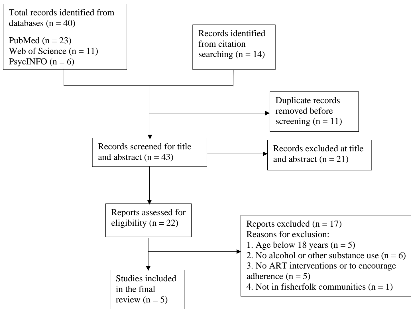
Fig. 1. PRISMA flow diagram
