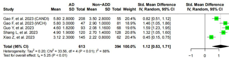
451 Figure 5. Forest plot of random effects meta-analysis of plasma p-tau181 levels in AD 452 and non-AD patients.
