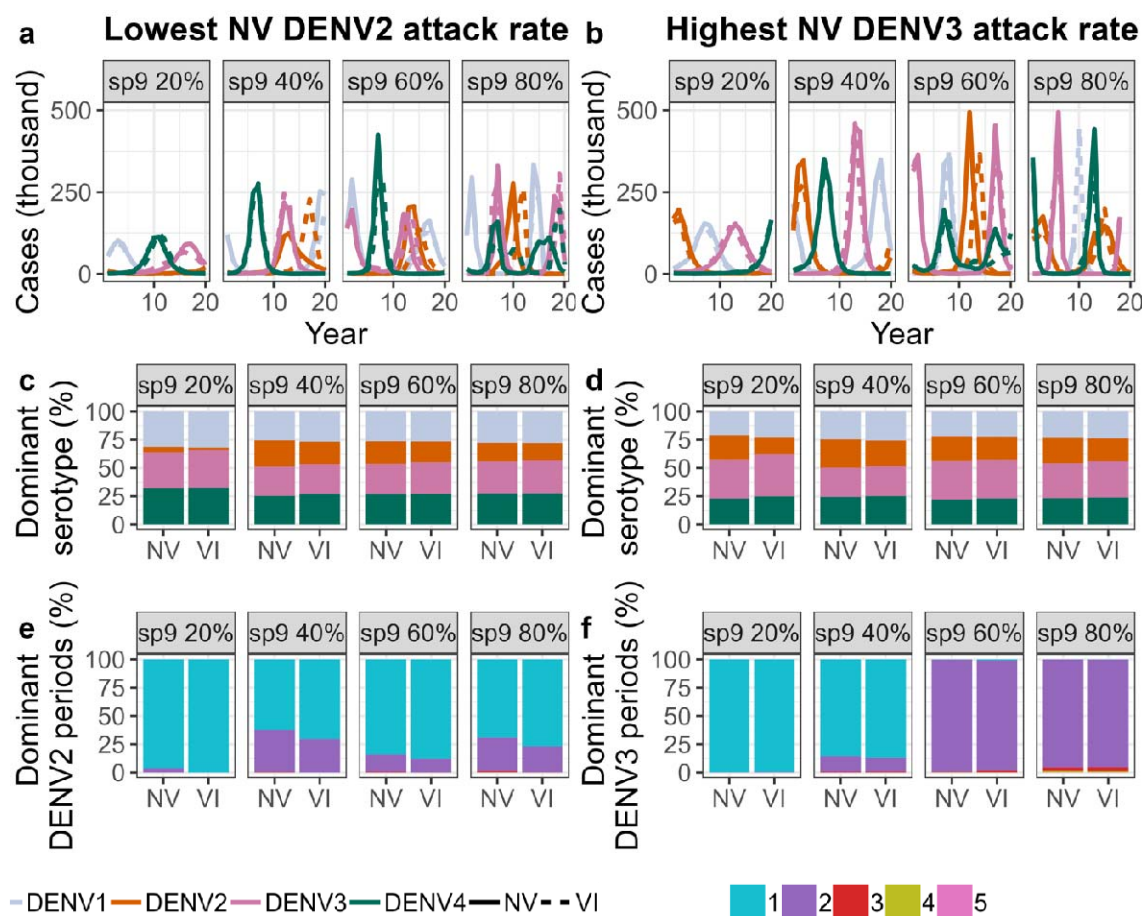
Figure 6: Impact of vaccination on serotype dynamics. For the 1,000 simulations with the lowest DENV2 burden (a, c, e) and the highest DENV3 burden (b, d, f), across transmission settings (sp9, average seroprevalence in 9-year-old) with (VI) and without (NV) vaccination we show (a-b) example serotype-specific transmission dynamics (c-d) the mean proportion of time each serotype is dominant and (e-f) the proportion of simulations (y-axis) in which DENV2 (e) and DENV3 (f) become the dominant serotype for the specified number of seasons (colours), over a 20 year period since the start of vaccination.
