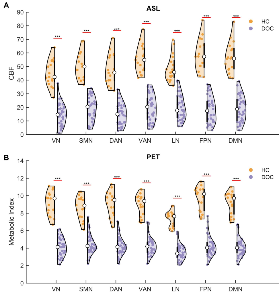
Fig.3 A) Unpaired t-test of CBF between HC and DOC in seven networks (FDR corrected, *** indicates p < 0.001 ). B) Unpaired t-test of metabolic index between HC and DOC in seven networks (FDR corrected, *** indicates p < 0.001 ).
