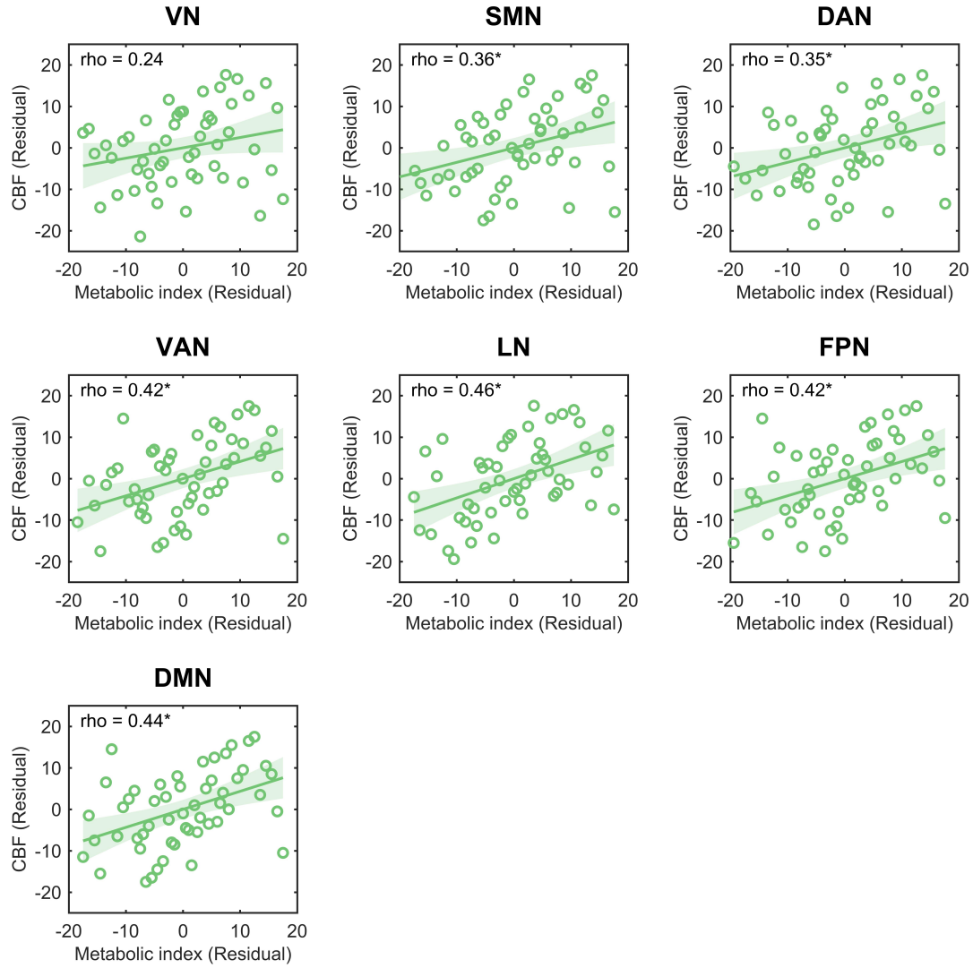
Fig.4 Spearman partial correlation between CBF and metabolic index across all participants in seven networks (two-tailed test, FDR corrected, * indicates p < 0.05 ).
