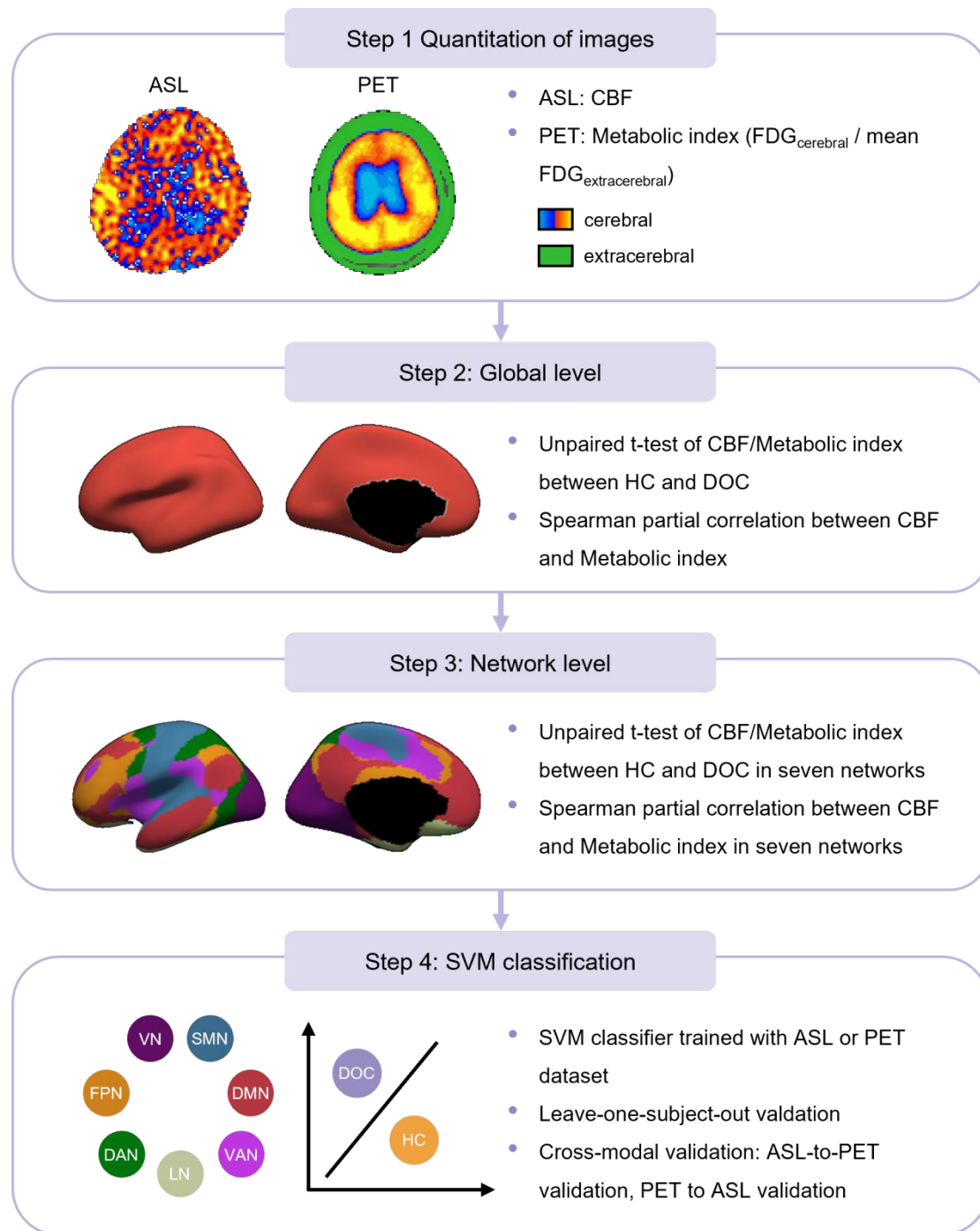
Fig.1 Flowchart of data processing procedure. Step 1 involves quantifying the images in both ASL and FDG-PET data. Step 2 involves comparing the cerebral blood flow (CBF) or metabolic index between HC and DOC groups at the global level, and performing Spearman’s partial correlation between the two modalities at the global level. Step 3 involves comparing the CBF or metabolic index between HC and DOC at the network level, and performing Spearman’s partial correlation between the two modalities at the network level. Step 4 involves model training and cross-validation for SVM classifiers. DMN = default mode network, FPN = frontoparietal network, LN = limbic network, VAN = ventral attention network, DAN = dorsal attention network, SMN = somatomotor network, VN = visual network.
