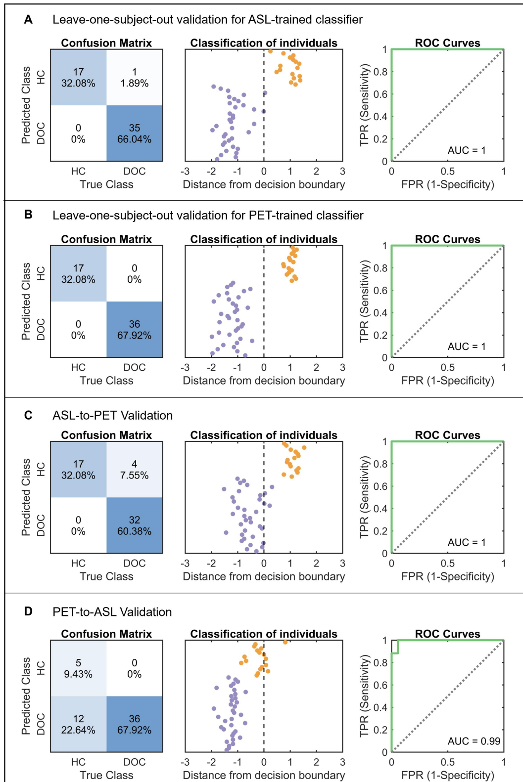
Fig.6 Performance of SVM classifiers trained with 100 features from 100 cortical regions. A) The ASL-trained and B) PET-trained classifiers were validated using leave-one-subject-out cross-validation. C) The ASL-trained classifier was validated with the normalized metabolic index from 100 regions in PET data. D) The PET-trained classifier was validated with the normalized CBF from 100 regions in ASL data. Confusion matrices, individual classification result and ROC curve are displayed for each validation. ROC = receiver operating characteristic; AUC = area under curve. TPR = true positive rate; FPR = false positive rate.
