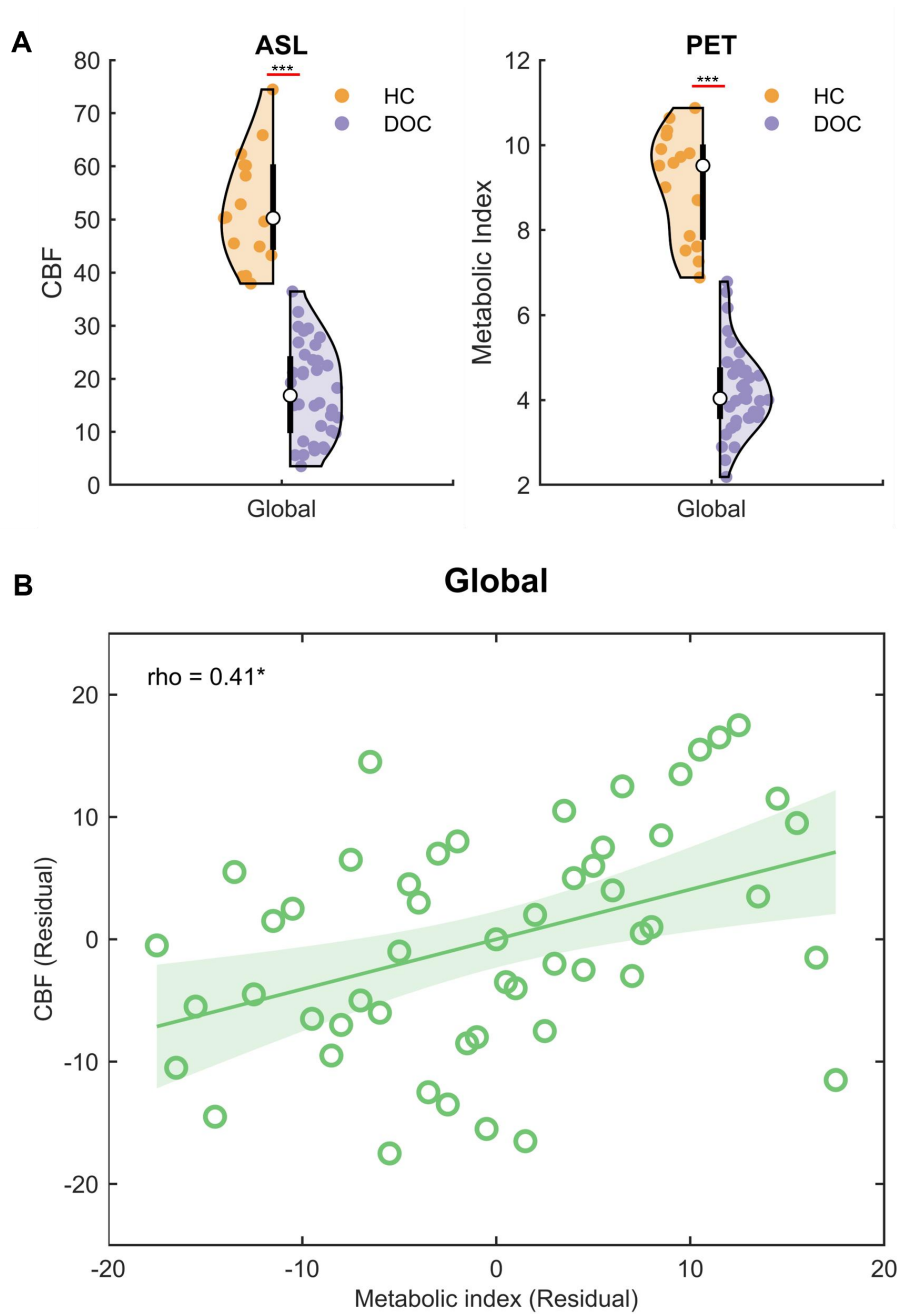
Fig.2 A) Unpaired t-test of CBF and metabolic index between HC and DOC in global gray matter (FDR corrected, *** indicates p < 0.001 ). B) Spearman's partial correlation between CBF and metabolic index across all participants in global gray matter (two-tailed test, FDR corrected, * indicates p < 0.05 ).
