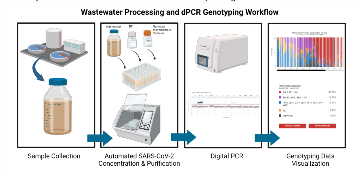
Figure 1: Workflow for wastewater processing and digital PCR genotyping. (1) Sample Collection: Untreated wastewater is collected from treatment facilities. (2) Automated SARS-CoV-2 Concentration & RNA extraction: Samples are concentrated using Nanotrap Microbiome A particles and extracted using MagMAX kit in a KingFisher Apex system. (3) Digital PCR: The samples are then analyzed to detect and quantify SARS-CoV-2 variants. (4) Genotyping Data Visualization: Data visualization shows the composition and prevalence of various SARS-CoV-2 variants over time.
