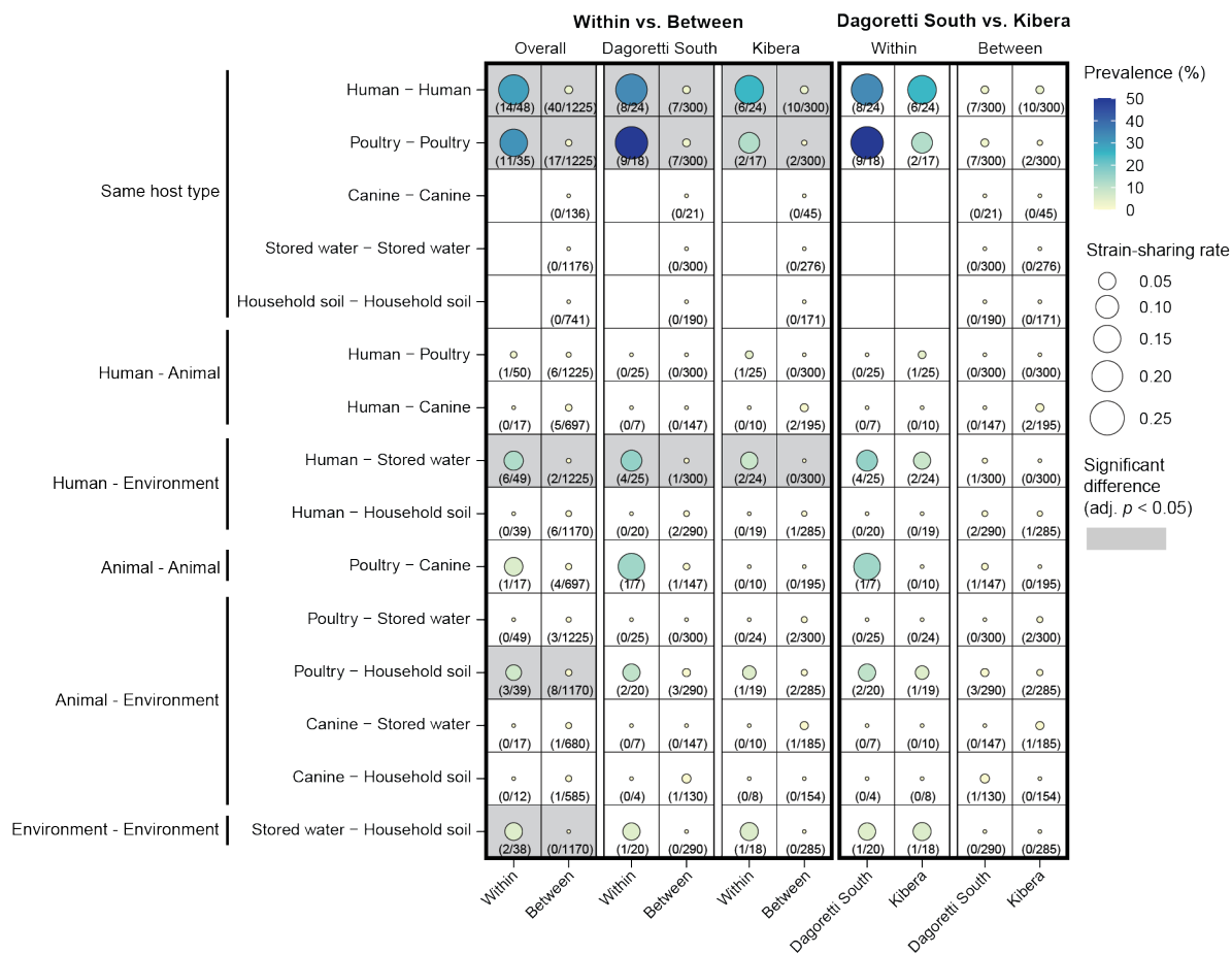
206 207 Fig. 3 Strain-sharing patterns within and between households. The size of each circle corresponds to the strain- 208 sharing rate (average strain-sharing events/total possible pairs in each household or household pair). The color gradient
