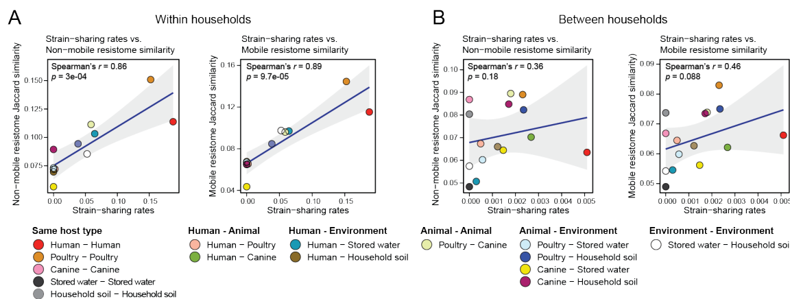
316 317 Fig. 6 Spearman's correlation analyses of non-mobile and mobile resistome similarity patterns with strain- 318 sharing patterns. Left and right panels are the analyses (A) within and (B) between households.
