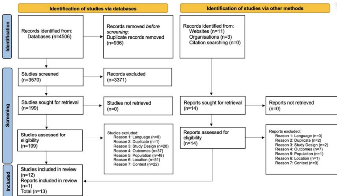
Figure 1. PRISMA flowchart
