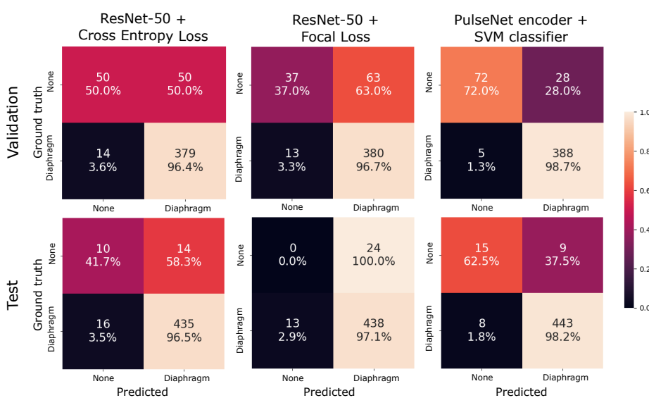
Fig. 2. Diaphragm detection confusion matrices.
