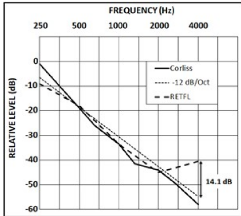
Figure 4. Normal bone-conduction thresholds from Corliss et al. (1959), a best-fit linear function with a slope of -12 dB/octave, and the bone-conduction RETFLs from ANSI S3.6-2018. The difference between the 4000 Hz RETFL and the best fit function is 14.1 dB, close to the false ABGs measured from listeners with SNHL. Values are relative levels (dB) from thresholds expressed in force units.
