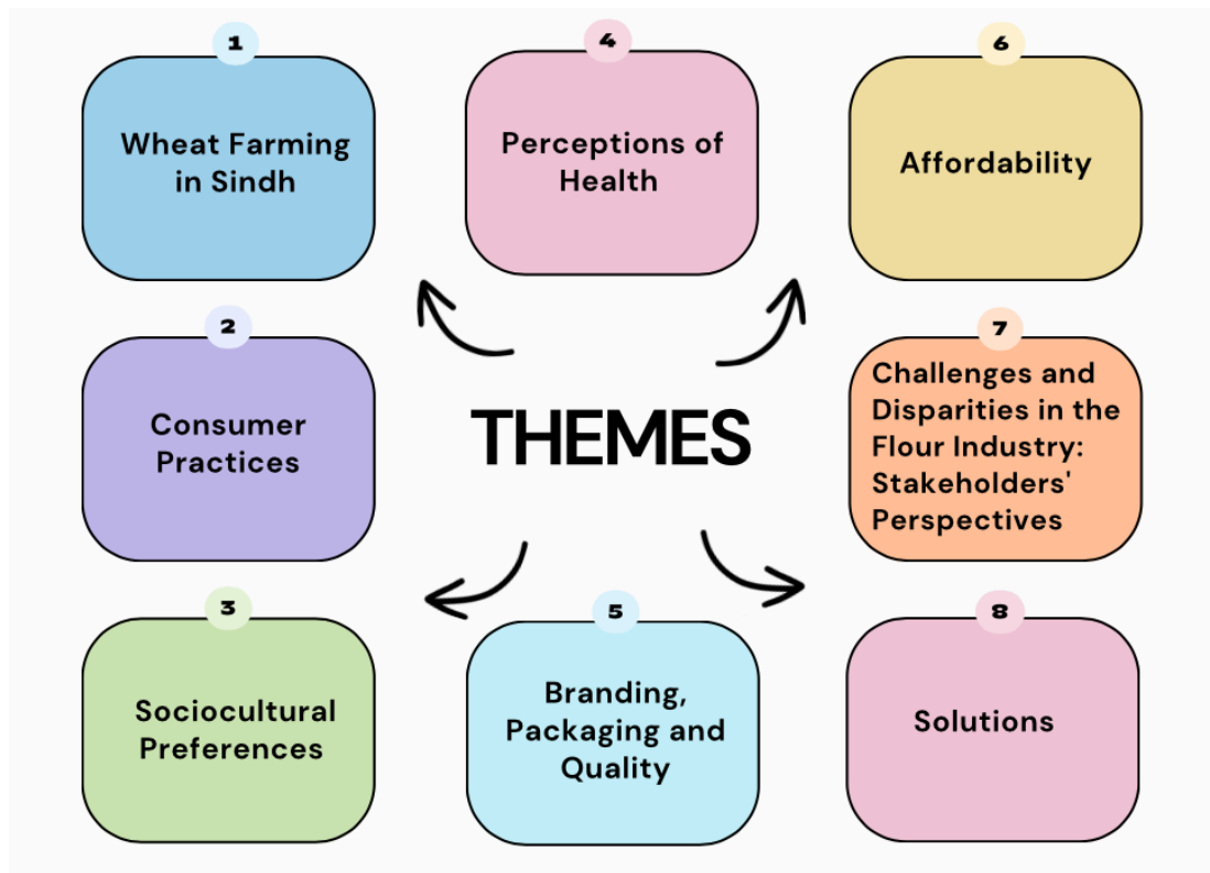
Figure 1: Themes
