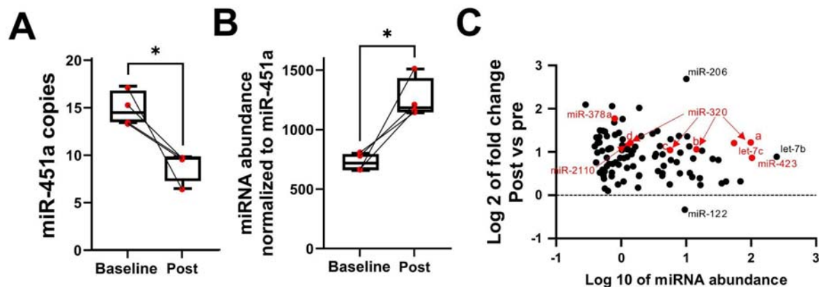
Figure 5. (A) CSF miR-451a decreases after Enoxacin treatment (B) Total CSF miRNA levels, normalized to miR-451a, in the CSF at baseline and at the completion of 1-month treatment with Enoxacin. * p < 0.05 , paired t-test. Data are presented as the mean \pm SEM of four patients per time point. (C) change in specific miRNA levels after 1-month treatment compared to baseline levels. miRNA counts in each sample were corrected to patients and normalized to the corresponding levels of miR-451a. Log 2 transformed fold change (y-axis) is shown against log 10 transformed mean miRNA abundance (x-axis). Red indicates significantly changed miRNAs (FDR < 0.1 , multiple paired t-test followed by the two-stage linear step-up procedure of Benjamini, Krieger and Yekutieli). miR-320 family members are shown with their suffix letter (a, b, c, d) next to the data point.
