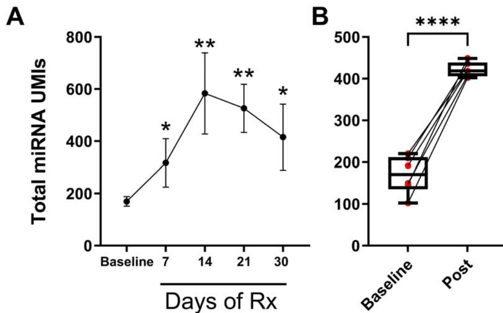
Figure 4. (A) Total miRNA levels, normalized by miR-451a levels in the plasma at baseline and on days 7, 14, 21 and 30 before morning dose (N=6 patients per time point). *FDR<0.1, **FDR<0.01 for comparisons vs baseline, Friedman test followed by Benjamini-Hochberg correction. (B) Total miRNA levels in the plasma, normalized to miR-451a, at baseline and post treatment (average of days 7, 14, 21 and 30). ***p<0.0001 vs baseline, paired t-test.
