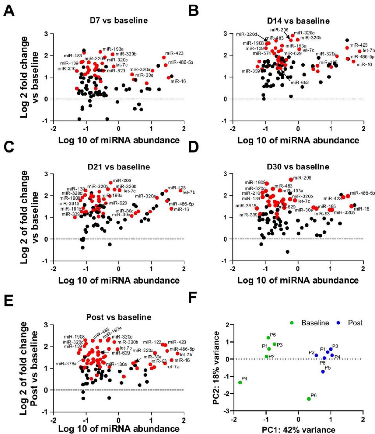
Figure 2. change in specific miRNA levels in the plasma, compared to baseline levels, on days 7 (A), 14 (B), 21 (C), 30 (D) and in all four time points averaged, compared to baseline (E). miRNA counts were corrected to patients and normalized to miR-451a levels. Log 2 transformed fold change (y-axis) is shown against Log 10 transformed mean miRNA abundance (x-axis). Red indicates miRNAs which are significantly changed vs baseline (FDR < 0.1 after multiple hypotheses correction). (F) principal component analysis of data presented in E by individual samples. Dots are annotated with the patient number. Green/blue dots denote baseline /post-treatment samples. Data in panels A-D were analyzed with two-way repeated measure ANOVA, data in E were analyzed with multiple t-tests. Multiple hypothesis correction was performed by a Two-stage linear step-up procedure of Benjamini, Krieger and Yekutieli.
