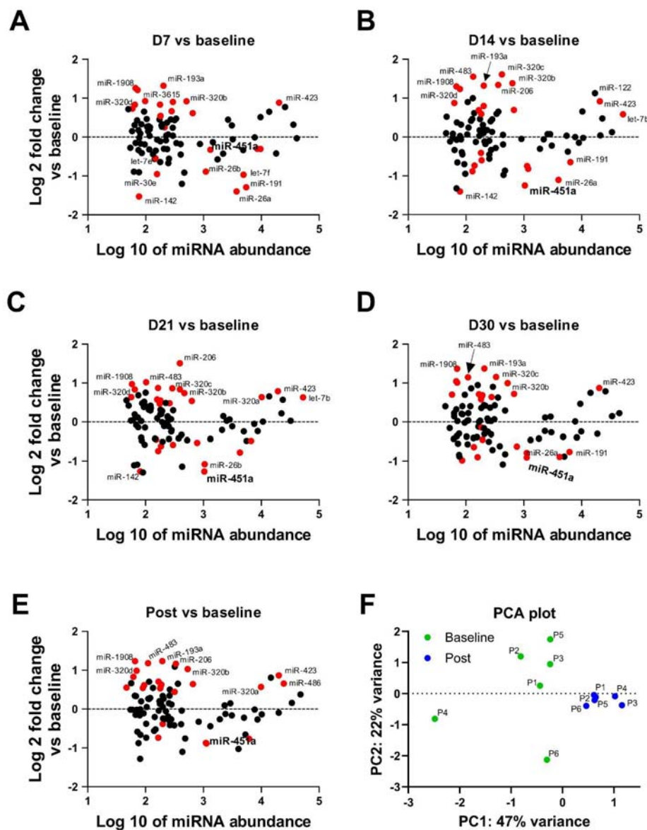
Supplementary figure 1. change in specific miRNA levels in the plasma, compared to baseline levels, on days 7 ( A ), 14 ( B ), 21 ( C ), 30 ( D ) and in all four time points averaged, compared to baseline ( E ). miRNA counts were corrected to patients and normalized to size factor by DESeq2. Log 2 transformed fold change (y-axis) is shown against Log 10 transformed mean miRNA abundance (x-axis). Red indicates miRNAs which are significantly changed vs baseline (FDR<0.1 after multiple hypotheses correction). ( F ) principal component analysis of data presented in E by individual samples. Dots are annotated with the patient number. Green/blue dots denote baseline/post-treatment samples. Data presented in panels A-D were analyzed with two-way repeated measure ANOVA. Data in E were analyzed with multiple t-tests. Multiple hypothesis correction was performed by a Two-stage linear step-up procedure of Benjamini, Krieger and Yekutieli.
