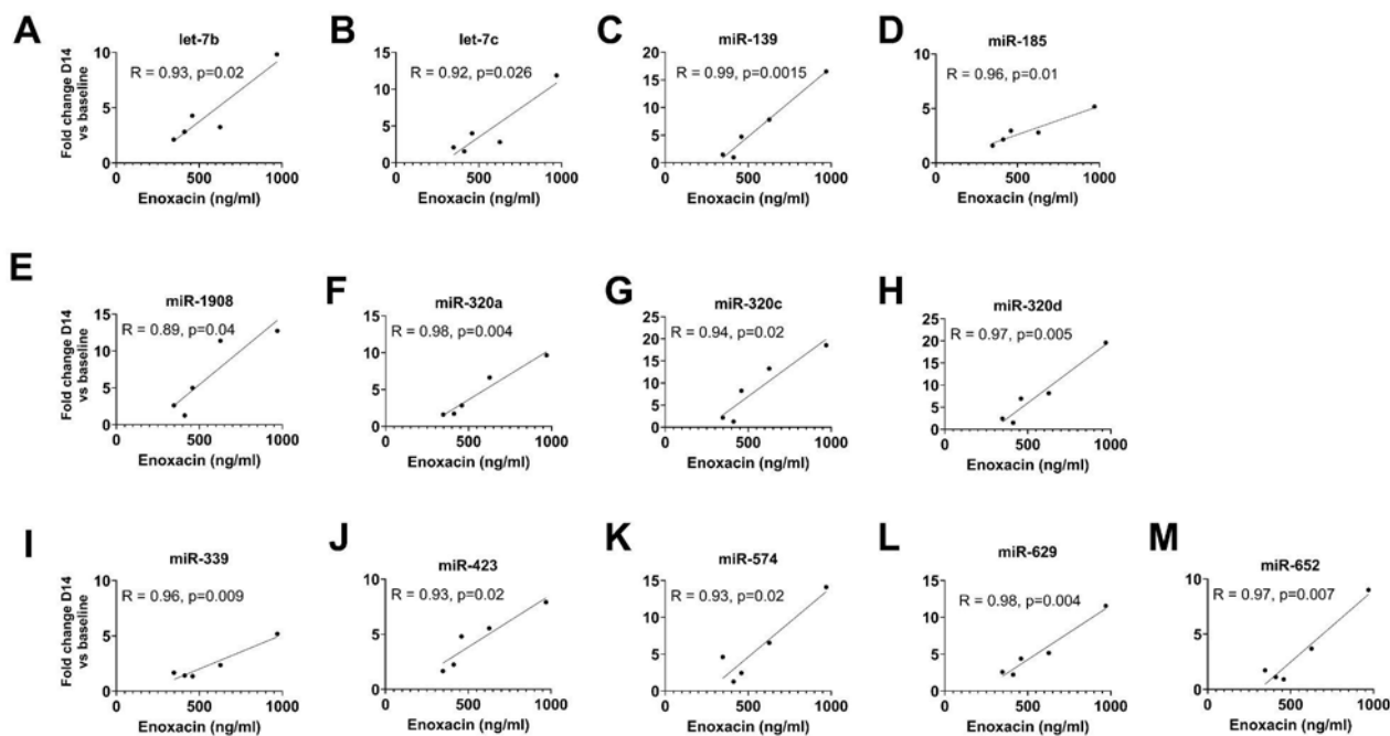
Figure 6. Pearson correlation between Enoxacin levels and fold-change values of miRNAs measured on day 14. p-values shown are unadjusted. All p-values displayed an FDR<0.1 after Benjamini-Hochberg correction.
