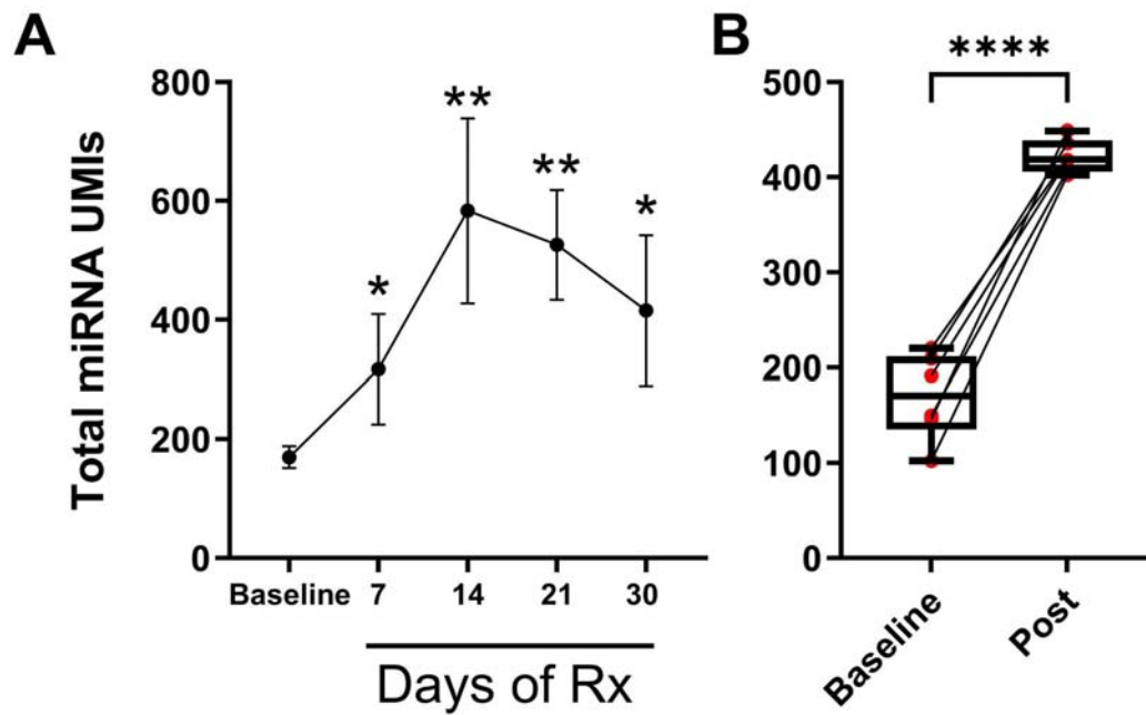
Figure 4. (A) Total miRNA levels, normalized by miR-451a levels in the plasma at baseline and on days 7, 14, 21 and 30 before morning dose (N=6 patients per time point). *FDR<0.1, **FDR<0.01 for comparisons vs baseline, Friedman test followed by Benjamini-Hochberg correction. (B) Total miRNA levels in the plasma, normalized to miR-451a, at baseline and post treatment (average of days 7, 14, 21 and 30). ***p<0.0001 vs baseline, paired t-test.
