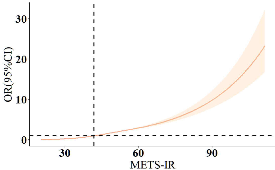
Figure 2: We conducted restricted cubic spline analysis to assess the association between METS-IR index and the risk of developing Type 2 Diabetes Mellitus (T2DM). The model was adjusted for all covariates. Odds ratios (OR) were depicted using a solid orange line, while the 95% confidence intervals were represented by a lightly shaded yellow area.
