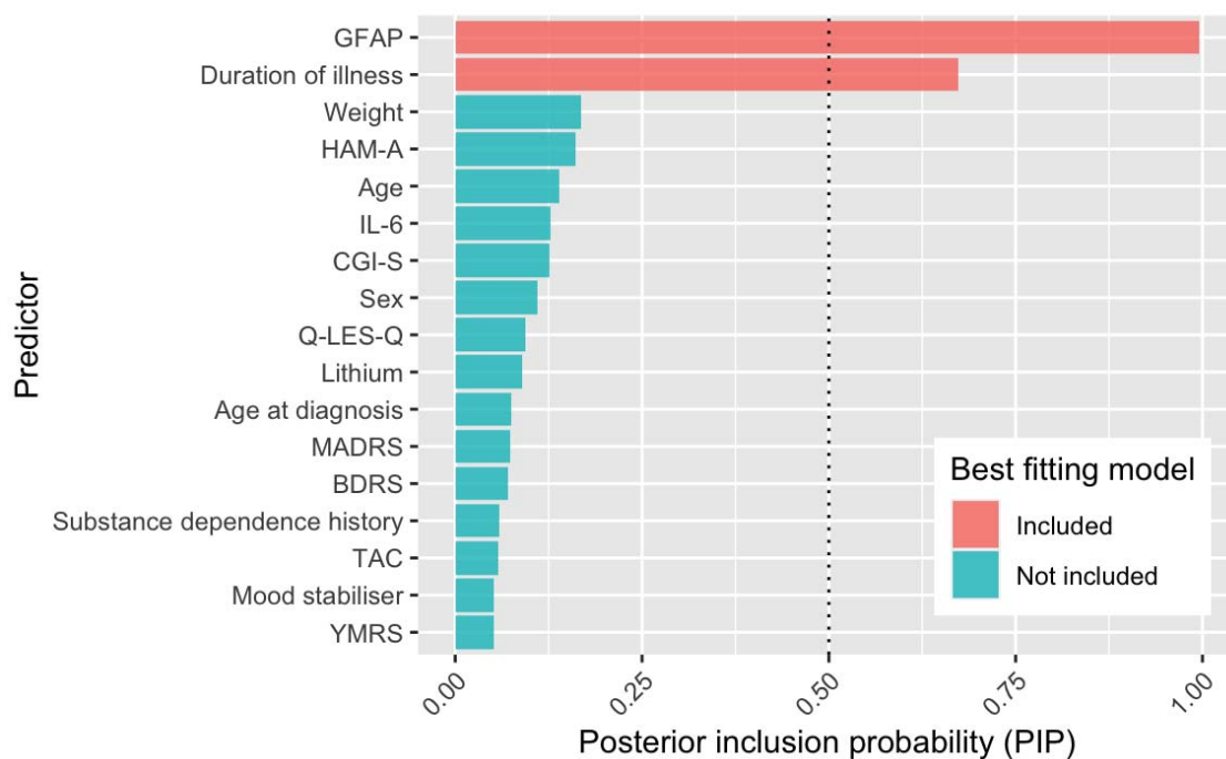
Figure 1a - PIP for each predictor of NfL and model parameters averaged across the model space.
