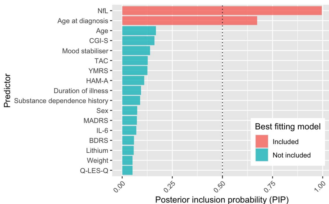
Figure 1b - PIP for each predictor of GFAP and model parameters averaged across the model space.
