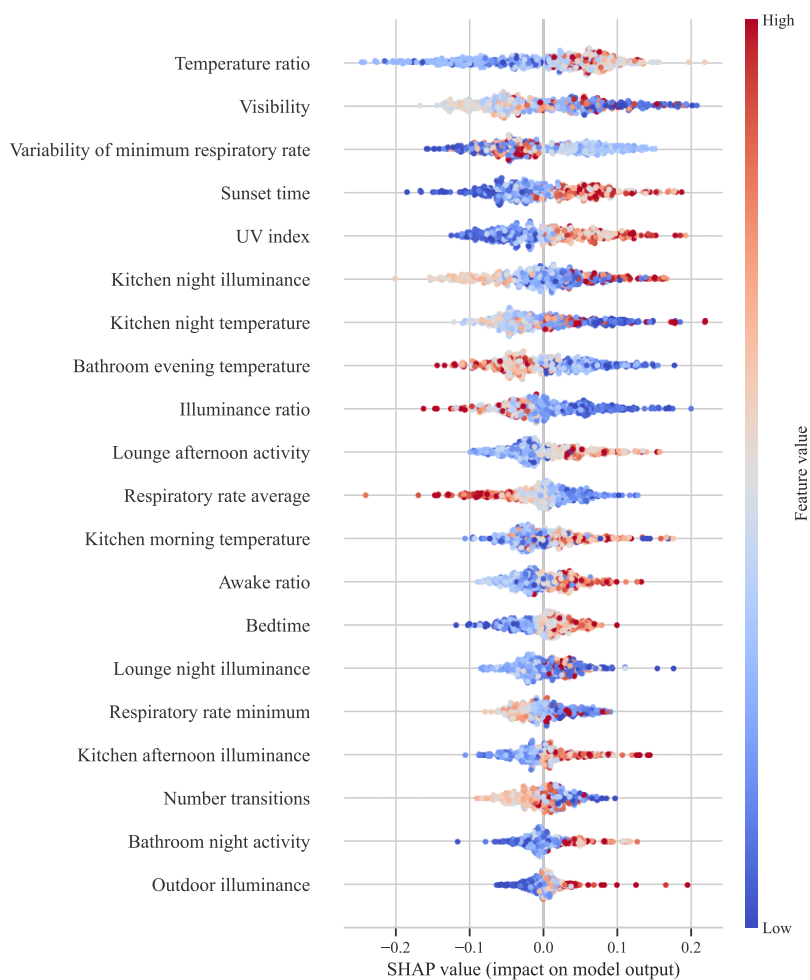
Figure 2: Model interpretability through feature importance analysis. The feature importance calculated using SHAP on the test sets from the 10-Fold cross-validation is shown in a summary plot. The colour represents the scaled feature value (red corresponding to higher values, blue to lower). The position of the x-axis represents the contribution of each normalised feature value to the positive prediction of agitation.
