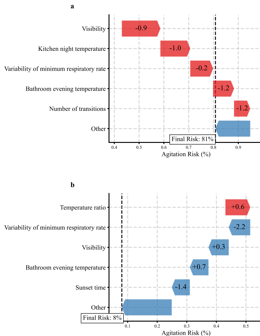
Figure 3: Personalised investigation of modifiable features. Examples from a positive (a) and a negative (b) event from PLwD A are shown using the SHAP framework. The colour of the arrow corresponds to the contribution: red contributes to agitation presence and blue contributes to agitation absence. Positive SHAP values contributed to positive predictions (agitated), while negative SHAP values contributed to negative predictions (non-agitated). The size of the arrow represents the absolute SHAP value, indicating the magnitude of each feature’s contribution. The number within the arrow corresponds to the normalised feature value.
