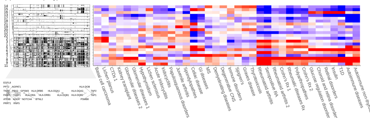
Figure 5: Haplotype group regression results. A dendrogram showing the clustering of the 40 most frequent haplotypes per haplotype group, with white representing the reference allele and black representing the effect allele. Genes are labeled below the corresponding SNPs overlapping their genome position, indicating which are within gene boundaries and which are intergenic. Heatmap showing the Z-scores from the haplotype group regression analysis across associated traits for A. Block 1 , B. Block 2 , and C. Block 3 , including all traits with at least one association |Z| > 4 in that block, and all haplotype groups with at least one trait association or total copies greater than the minimum cutoff of 20,000 copies. For visualization purposes, traits are clustered and Z-scores were set to a maximum of |Z| of 5.
