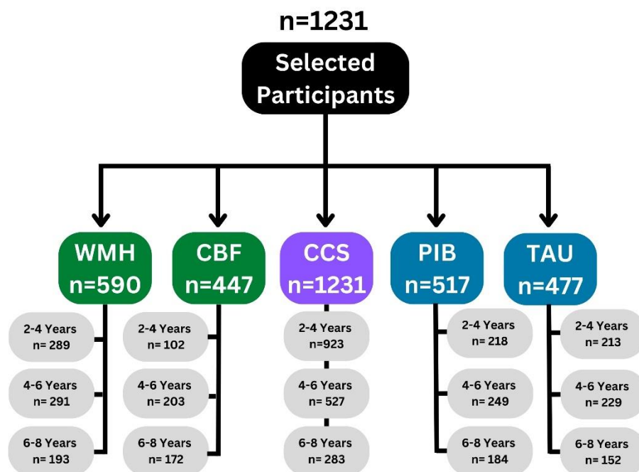
Figure 1: Sample sizes for the outcomes and time period between the predictor and outcome.
