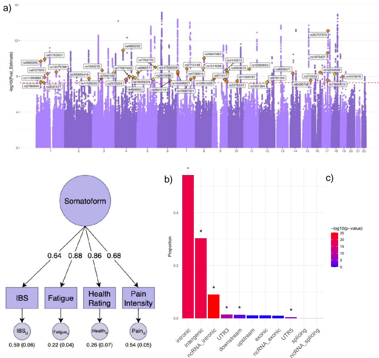
Figure 2. GWAS results for the somatoform factor.
