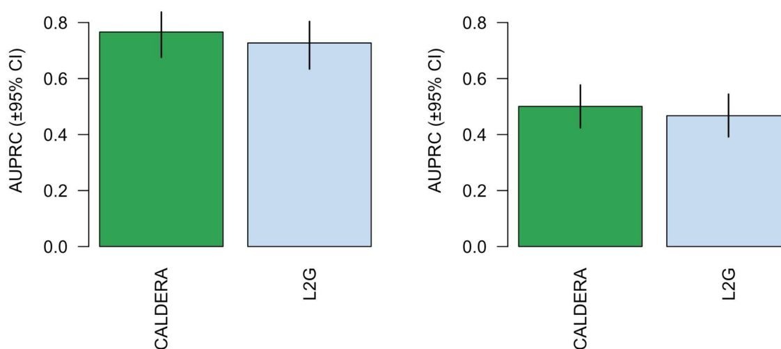
Figure 5. Area under the precision-recall curve ( \pm 95\% confidence intervals) for CALDERA and L2G model predictions in A ) the Open Targets ground truth dataset or B ) a ground truth dataset derived from burden tests of rare coding variants in the UK Biobank.
