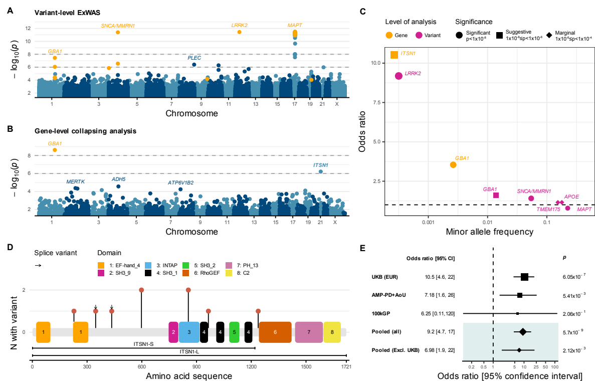
Figure 2. Variant- and gene-level associations with PD (A, B) Manhattan plots of variant-level (A) and gene-level (B) associations with PD in UKB Europeans. For each plot, if the same association was detected in multiple models, we depict the most significant association. See Figures S2, S4 for per-model plots. Horizontal dashed lines indicate the significance ( p < 1 \times 10^{-8} ) and suggestive ( p < 1 \times 10^{-6} ) thresholds. Orange points indicate marginally significant ( p < 1 \times 10^{-4} ) associations in genes previously implicated in PD. (C) Odds ratio versus minor allele frequency for ITSN1 and other established PD loci that achieved p < 1 \times 10^{-4} in the ExWAS or collapsing analysis. (D) Lollipop plot showing the location of ITSN1 PTVs in cases against the MANE transcript (ENST00000381318) and Pfam domains of the corresponding protein (Q15811); bars
