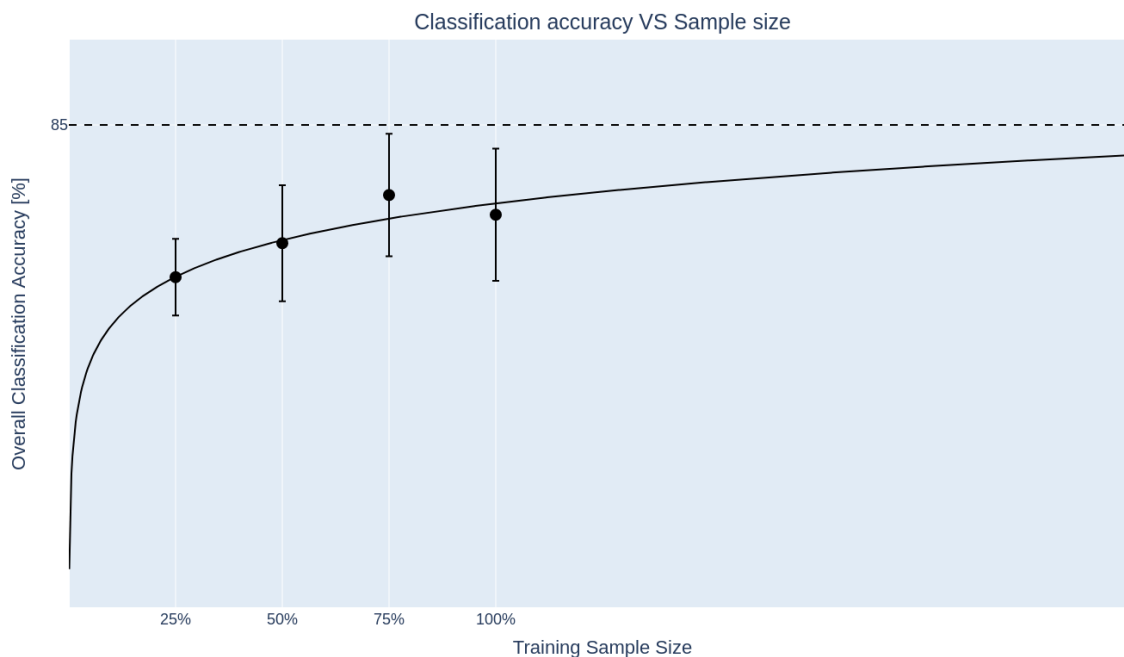
Figure 2 - Classifier power curve.
