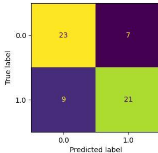
Figure 1 - Confusion matrix of the LOO classification on the CLM dataset
