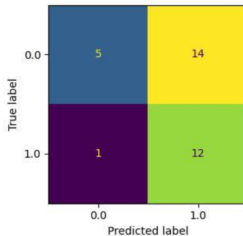
Figure 3 - Confusion matrix of the DRAMA-BPD classification on the MEX dataset.
