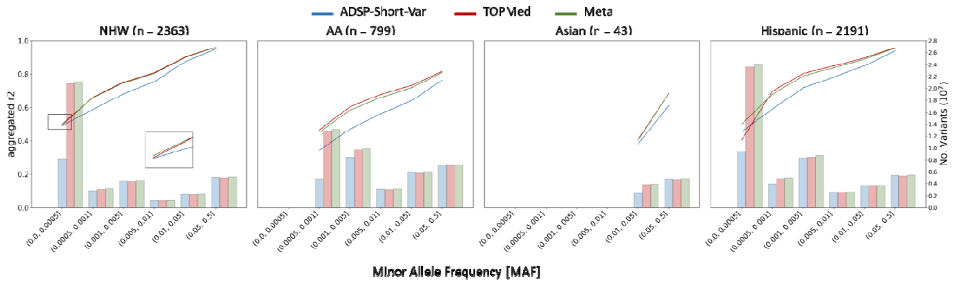
209 210 Figure 2. Comparison of aggregated R^2 , the squared Pearson correlation between genotypes obtained 211 from imputations and WGS, for four ethnicities. The bars indicate the total number of variants 212 analyzed for each ethnicity.
