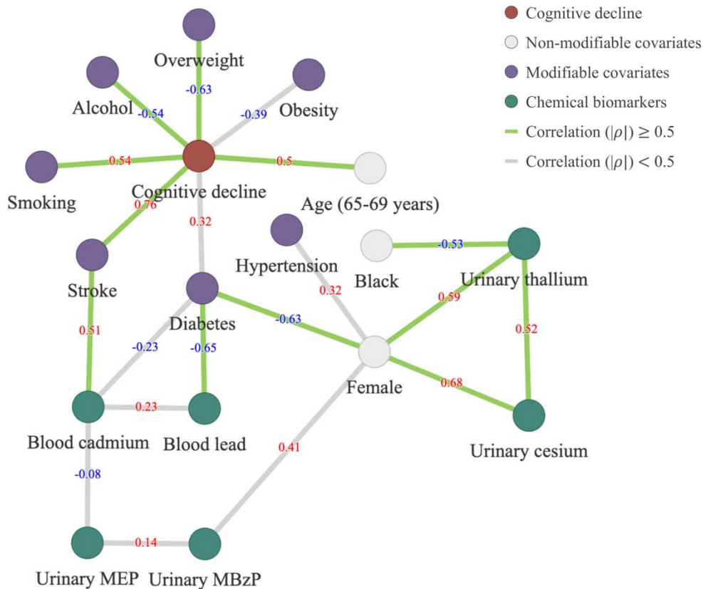
288 289 Figure 3. Partial correlation ( ) network plot depicting the magnitude and direction of 290 correlation coefficients among identified chemical biomarkers, cognitive decline, and selected 291 covariates. Only chemical biomarkers or covariates with significant correlation coefficients with 292 cognitive decline (adjusted p -value < 0.05 ) are shown. Green lines indicate relatively strong 293 correlation coefficients ( |\rho| \geq 0.5 ). Red numbers indicate positive correlations and blue numbers 294 indicate negative correlations.
