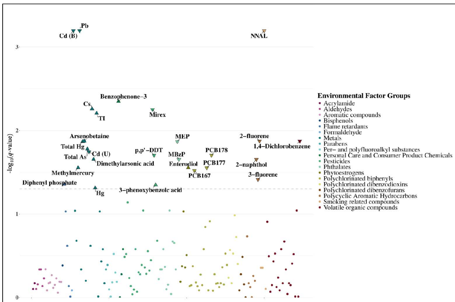
238 239 Figure 2. Manhattan plot of environmental factors (chemical biomarkers) associated with the Digit Symbol Substitution Test (DSST) 240 z-scores. Significant chemical biomarkers were dotted above the grey dashed line ( q -value < 0.05 ), and the arrows indicated the 241 direction of their effects on DSST z-scores. Abbreviation: B, blood; DDT, dichlorodiphenyltrichloroethane; NNAL, 4- 242 (methylnitrosamino)-1-(3-pyridyl)-1-butanol; PCB, polychlorinated biphenyl; U, urine.
