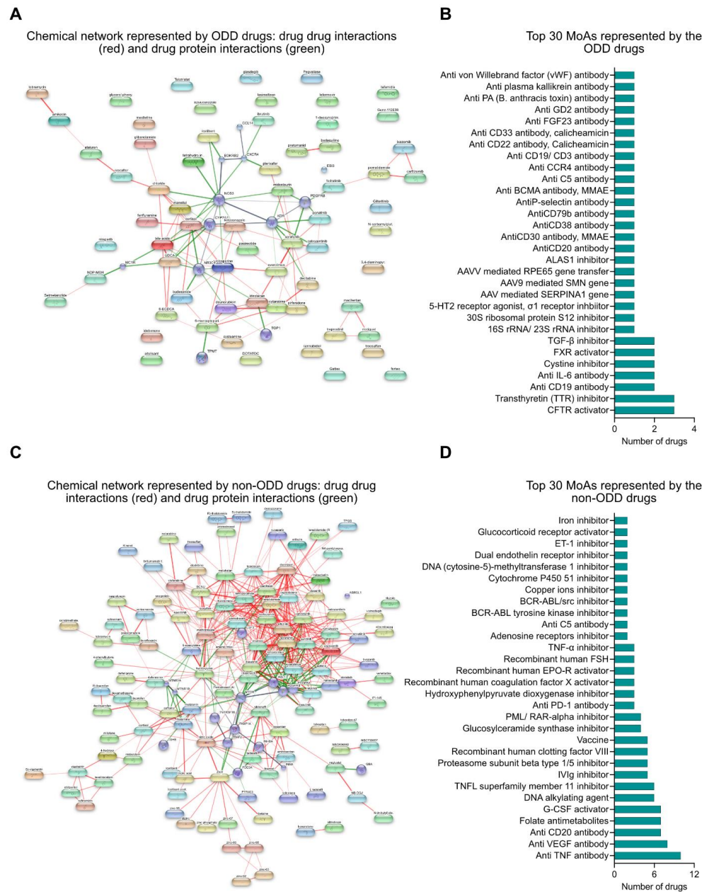
Figure 4: (A) Chemical network represented by ODD designated interventions: drug-drug (red) and drug-protein (green) interaction framework. (B) Top 30 mechanisms of actions represented by interventions with ODD designation. (C) Chemical network represented by non ODD interventions: drug-drug (red) and drug-protein (green) interaction framework. (D) Top 30 mechanisms of actions represented by interventions without ODD designation.
