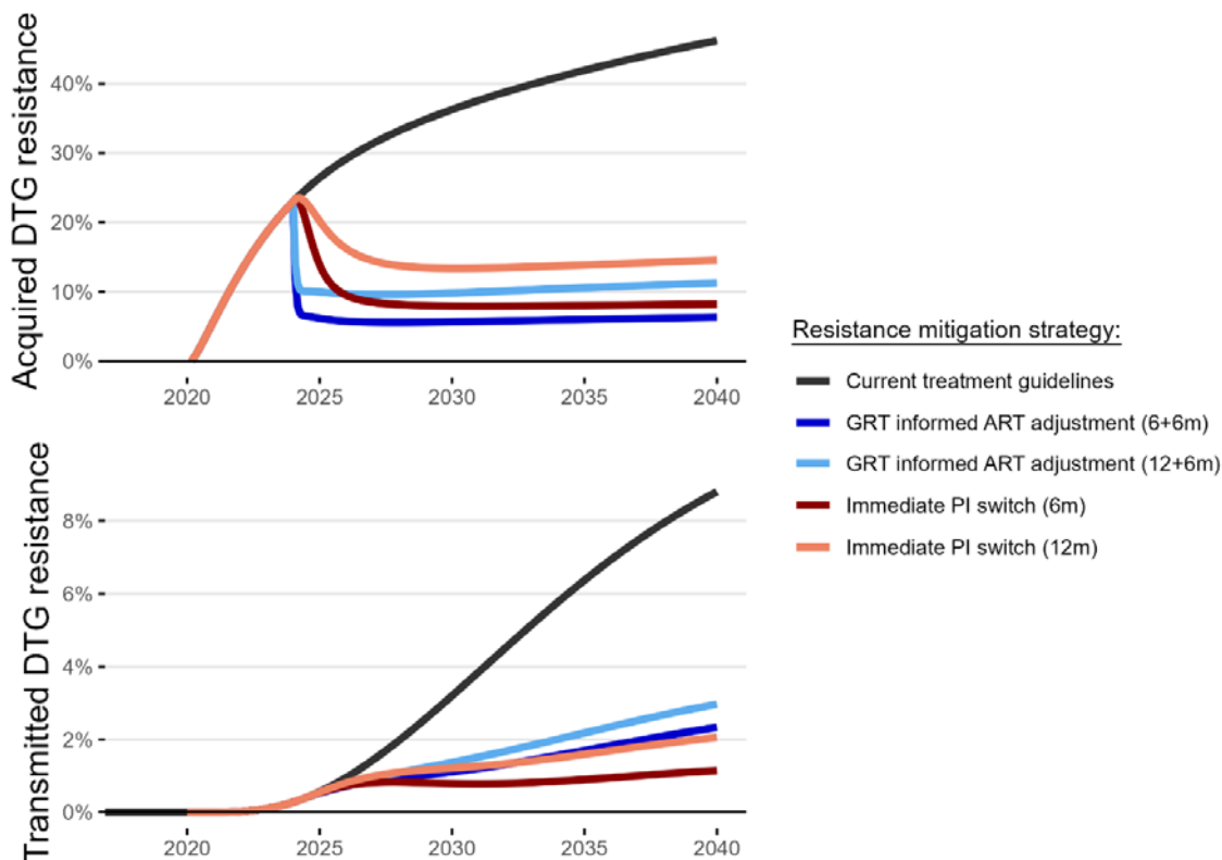
Figure 3: Counterfactual scenario, modelling resistance emergence mitigation strategies. Both strategies reduce the duration with viremia on dolutegravir-based ART. GRT-informed ART adjustment includes druglevel testing and genotypic resistance testing upon detecting virologic failure, followed by switching to PI-based ART in case of intermediate or high level dolutegravir resistance. Immediate PI switch includes switching people with virologic failure on dolutegravir-based ART immediately to PI-based ART. Modelled scenarios include projections assuming 6 and 12 months until virologic failure is detected (6 months: dark blue and dark red lines; 12 months: light blue and light red lines) upon which the respective strategy is implemented immediately. In case of druglevel and genotypic resistance testing, we assume an additional average duration of 6 months from detection of virologic failure to informed treatment adjustment. Acquired dolutegravir resistance is defined as proportion of people on a failing dolutegravir-based ART with intermediate- or high-level dolutegravir resistance. Transmitted dolutegravir resistance is defined as proportion of newly diagnosed people with intermediate- or high-level dolutegravir resistance..
