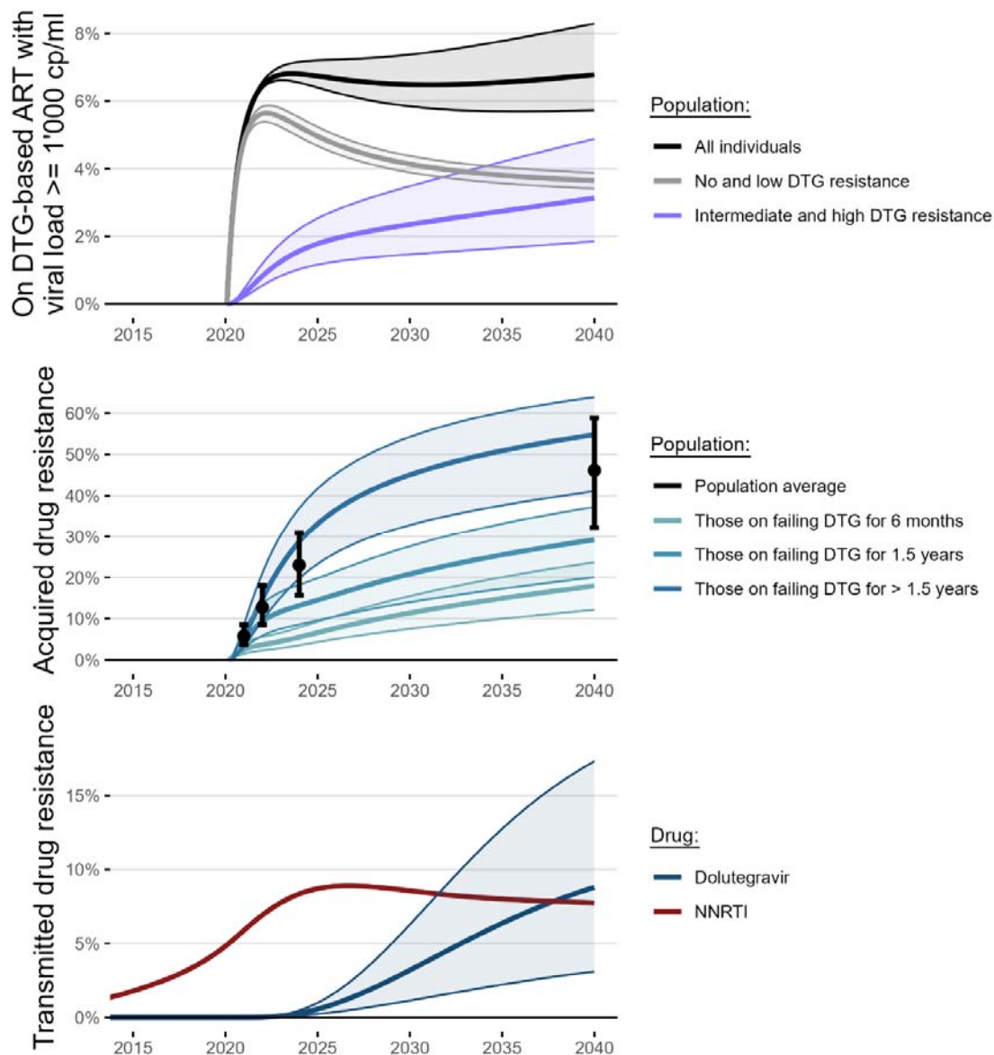
Figure 2: Modelled viral suppression on DTG-based ART, acquired and transmitted dolutegravir resistance. Solid lines show baseline parameterisation regarding mutation reversion rates, impact of NRTI resistance on dolutegravir DRM acquisition, impact of dolutegravir resistance on its efficacy, transmission probability of dolutegravir DRMs in an HIV transmission event, and proportion with detectable drug levels on failing dolutegravir-based ART. Shaded areas correspond uncertainty intervals (see appendix p12). Dolutegravir rollout was started in 2020. Viral suppression (viral load below 1'000 copies per ml) on dolutegravir-based ART is high; depending on the model assumptions for dolutegravir resistance (see uncertainty range), between 6% and 8% of people on dolutegravir-based ART may be virally unsuppressed. Acquired dolutegravir resistance is defined as proportion of people on a failing dolutegravir-based ART with intermediate- or high-level dolutegravir resistance. Transmitted dolutegravir resistance is defined as proportion of newly diagnosed people with intermediate- or high-level dolutegravir resistance.
