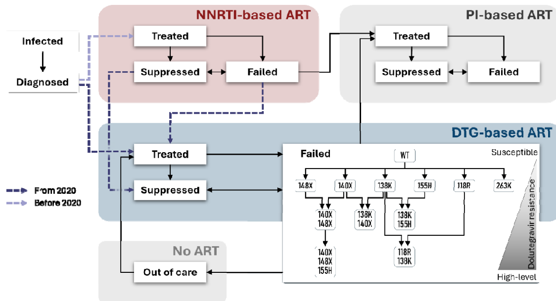
Figure 1: Simplified schematic overview of the adapted MARISA model. The treatment dimension, including dolutegravir resistance acquisition on failing dolutegravir-based ART, is shown. Not displayed here are the dimensions for gender and CD4 levels, NNRTI- and NRTI resistance acquisition, and mortality. Details on the model structure can be found in the appendix p3-11.
