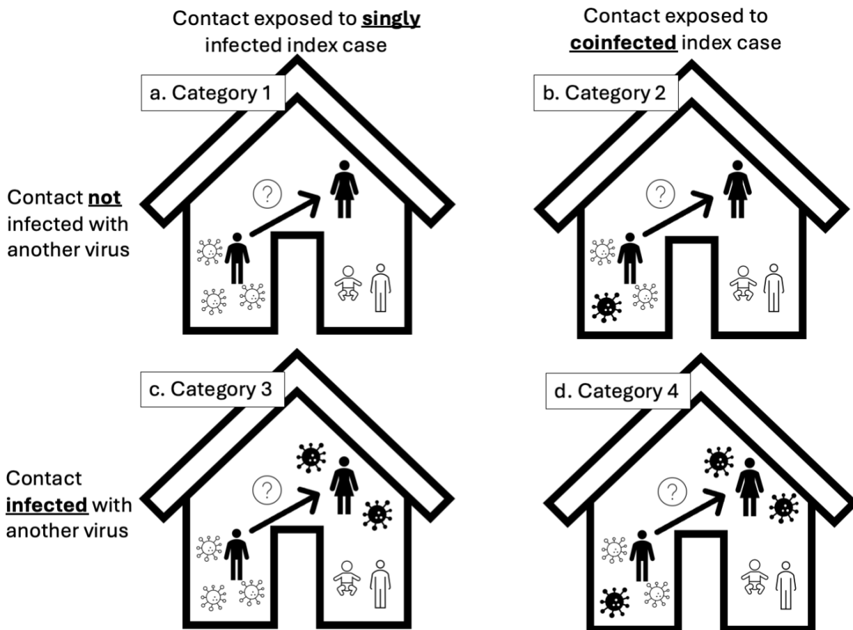
Figure 1. Four-category exposure variable used in multivariable mixed effects logistic regression models
