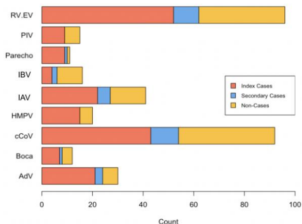
Figure 2. Viruses detected during household illness events, by primary virus of interest AdV = adenovirus, Boca = bocavirus, cCoV = common/seasonal coronaviruses, HMPV = human metapneumovirus, IAV = influenza A virus, IBV = influenza B virus, Parecho = parechovirus, PIV = parainfluenza virus, RSV = respiratory syncytial virus, RV.EV = rhinovirus/enterovirus *Non-cases are those who were involved in a household illness cluster event for a virus of interest and did not test positive for the virus of interest.
