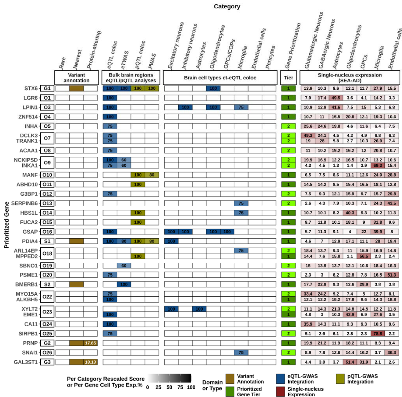
Figure 1. Gene prioritization results for sCJD GWAS. A visual summary of weighted evidence category scores for each prioritized risk gene, together with brain cell-type-specific gene expression proportions. The figure shows a total of 32 prioritized risk genes (17 tier 1 and 15 tier 2). The leftmost squares indicate the locus indexes where “G” is used for the genome-wide significant loci, “S” for the subthreshold loci, and “O” for the remaining other loci. The types of evidence for each category are coloured according to the three different domains to which they belonged. Weighted scores for each evidence category are rescaled to a 0–100 scale based on the maximum score a candidate gene can obtain from a category (see Supplementary Table 3 ). The darker colours represent higher scores in categories or higher average gene expression proportions in the 7 major brain cell types, while tier 1 prioritized genes are displayed in dark green and tier 2 prioritized genes are displayed in light green. Only tier 1 and tier 2 genes are shown for each locus, and all candidate genes considered and scored can be found in Supplementary Table 4 . CADD (v1.7) PHRED scores for index variants are labelled in white within the respective squares in variant annotation domain. eQTL, expression QTL; pQTL, protein-expression QTL; ct-eQTL, cell-type-specific eQTL; coloc, colocalization; TWAS, transcriptome-wide association study; PWAS, protein-wide association study.
