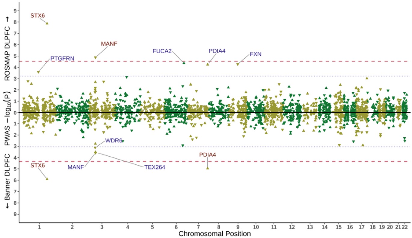
Figure 3. sCJD brain proteome-wide association study results. sCJD brain proteome-wide association study (PWAS) results are shown proteome-wide for both of the PWAS reference panels with two mirrored Manhattan plots on the x-axis; the upper side of the plot displays the results for ROSMAP DLPFC PWAS, while the lower side of the plot displays the results for Banner DLPFC PWAS. Proteome-wide significance thresholds (0.05 divided by number of tested associations) for both analyses are indicated with red dashed lines and suggestive significance thresholds (1 divided by number of tested associations) with a blue dotted line, and all the genes whose protein products are passing these thresholds are labeled, and colored based on their significance (red: proteome-wide significant, blue: suggestive significant). The directionality of Z-scores of each PWAS association are represented with up-pointing triangles (positive Z-score) and down-pointing triangles (negative Z-score). y axis, -\log_{10} PWAS P ; x axis, GRCh38 chromosomal positions. DLPFC, dorsolateral prefrontal cortex.
