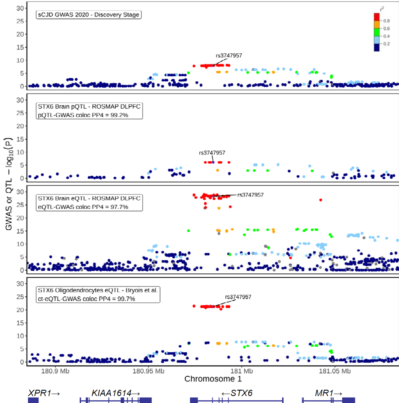
Figure 2. Regulation of STX6 brain gene and protein expression by the sCJD-risk-colocalized eQTLs and pQTLs within the STX6 locus. The regional plots of (i) sCJD GWAS association signal ( n = 17,679 ), (ii) STX6 brain pQTL signal in DLPFC (ROSMAP DLPFC pQTL catalogue, n = 376 ), (iii) STX6 bulk brain eQTL signal in DLPFC (ROSMAP DLPFC eQTL catalogue, n = 560 ), and (iv) STX6 ct-eQTL signal in oligodendrocytes (Bryois et al. 24 ct-eQTL catalogue, n = 192 ) are shown for 100 kb extended genomic coordinates of the STX6 locus index variant rs3747957 (chr1:180884717-181084717). Boxes in each panel shows QTL-GWAS coloc PP4 values between the molecular QTL signal and the GWAS signal for all tested variants (see Supplementary Tables 5-6 ). The index variant is shown in purple, and LD r^2 values (calculated within 1 KG non-Finnish European samples [ n = 404 ] with respect to the index variant) are indicated on a color scale, and variants that are not available in the
