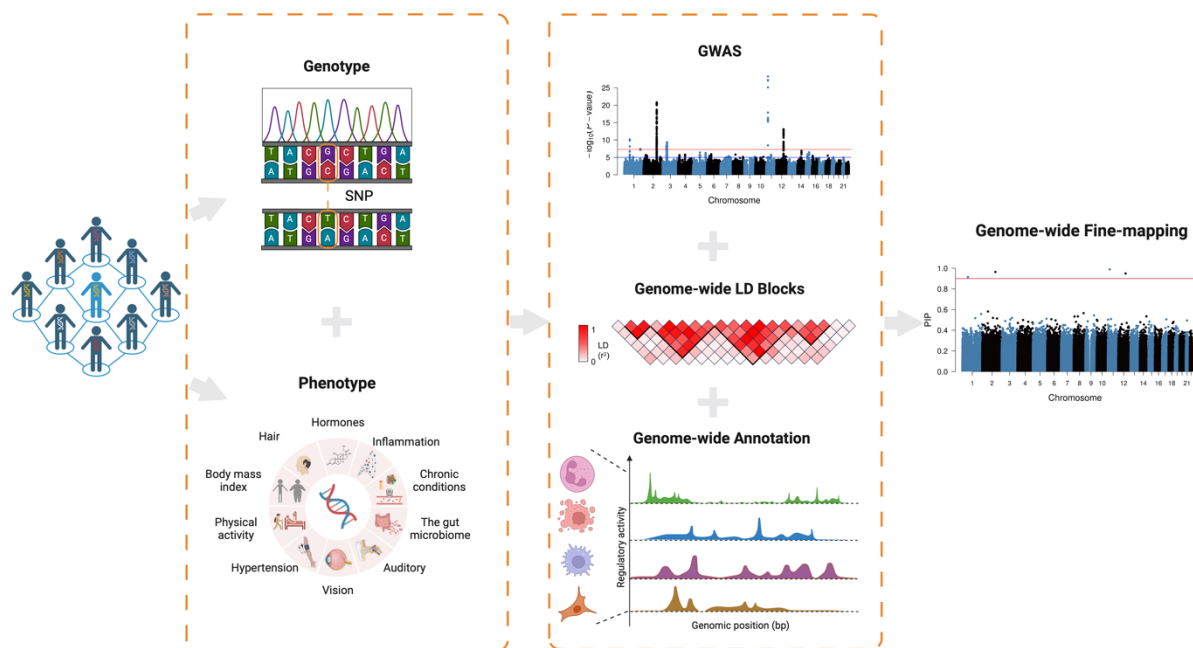
960 961 Figure 1 Schematic overview of genome-wide fine-mapping analysis using GBMM. GBMM 962 requires the GWAS summary statistics and genome-wide LD reference to fine-map the likely 963 causal variants for complex traits, and can incorporate functional annotations. Compared to 964 regional-based fine-mapping approaches, GBMM estimates priors with genome-wide SNPs and 965 MCMC sampling algorithm, and is more flexible on the assumption of the underlying distribution 966 of causal effects ( Table S1 ). The illustration was created with BioRender.com.
