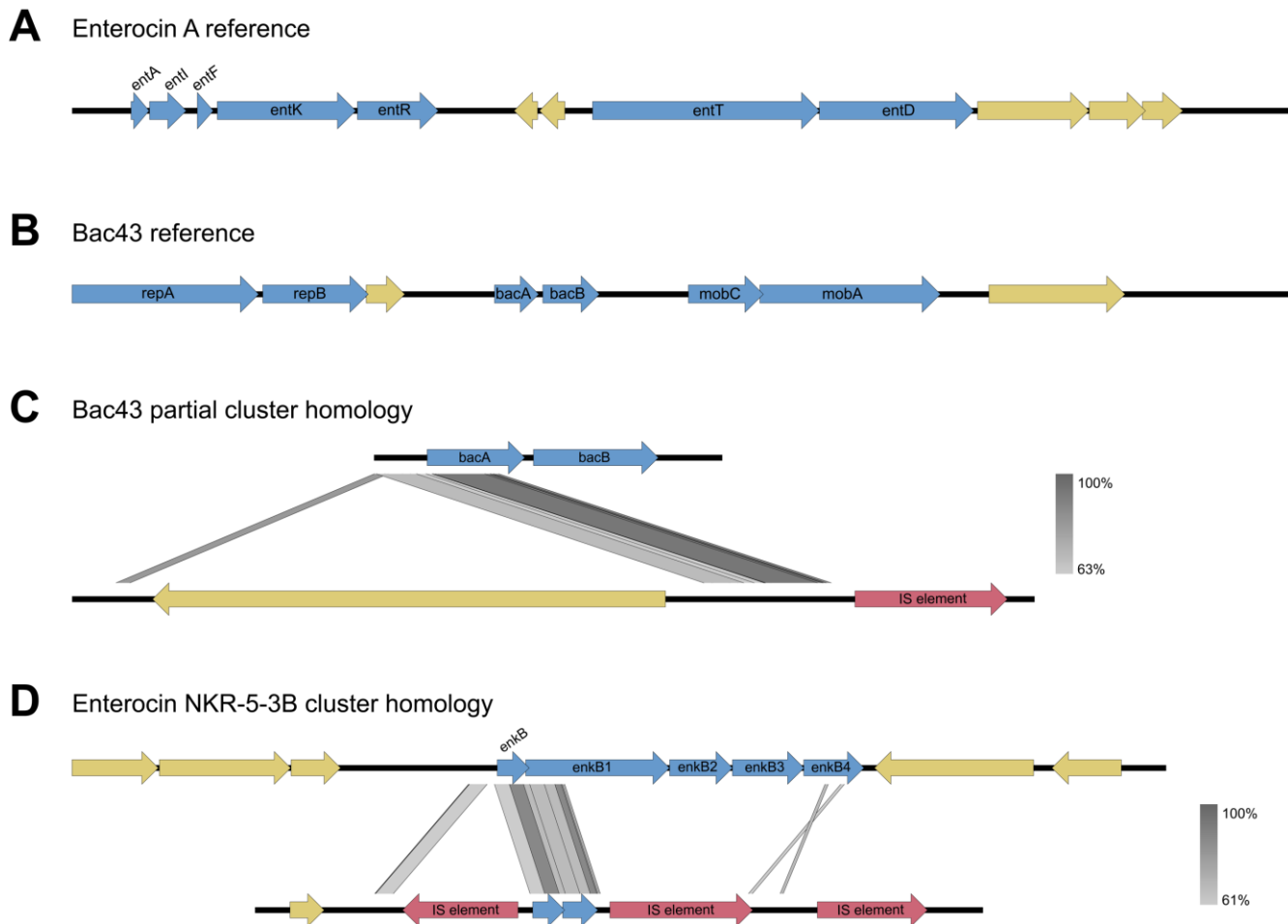
Figure 2: Gene maps and homology to previously identified bacteriocins. Genes related to bacteriocin production are blue, hypothetical proteins are yellow, and insertion elements are red. A. Internal reference of the enterocin A gene cluster. B. Internal reference of the bacteriocin 43 encoding plasmid pDT1. C. Homology of the bacteriocin 43 genes to the bac43 partial cluster BLAST hit. D. Homology of the enterocin NKR-5-3B genes to the enterocin NKR-5-3B cluster BLAST hit.
