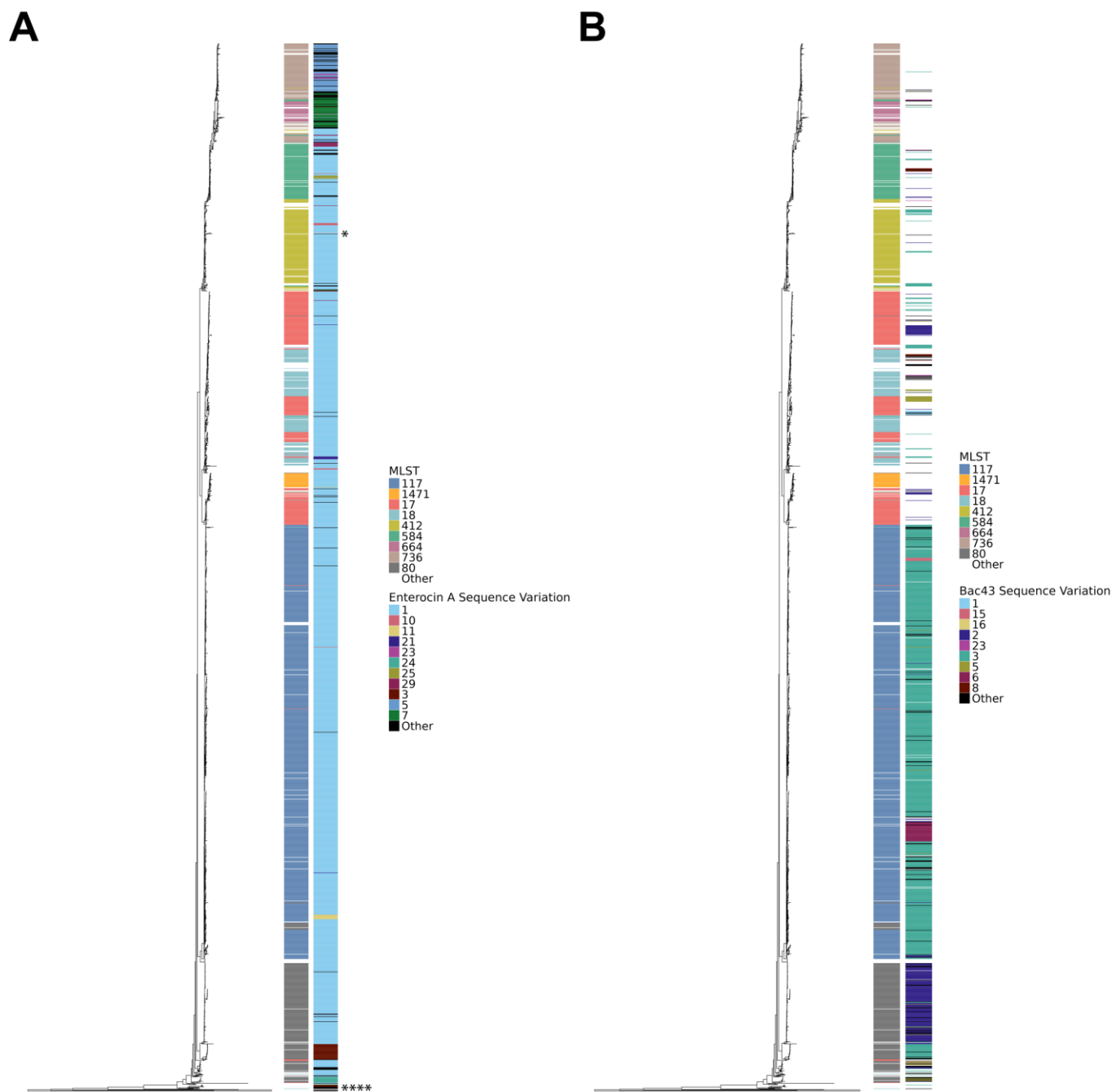
Figure 7: Phylogenetic mapping of bacteriocin genotype and phenotype. Core genome phylogeny with recombination removed by Gubbins. Outermost heatmap represents the bacteriocin sequence. Sequences with less than five isolates are classified as “Other.” Innermost heatmap is the isolate’s MLST. MLSTs with less than 20 isolates are classified as “Other.” A. Enterocin A sequences. Enterocin A isolates with the full enterocin A locus and an inhibitory phenotype are each indicated by an “*” B. Bac43 sequences.
