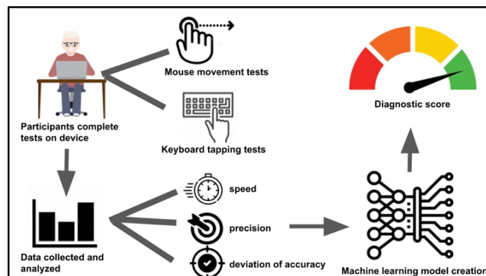
Figure 1. Pipeline for developing the core AI model used in this study. Mouse and keyboard data are collected from participants, a series of features are derived from the raw data, and these features are fed as input into a machine learning model which performs the prediction of PD vs. no PD.
