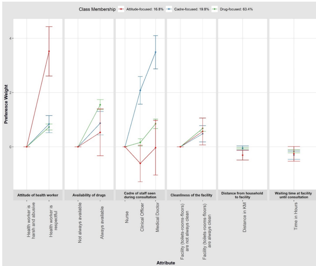
373 Figure 3: Latent Class Model results
