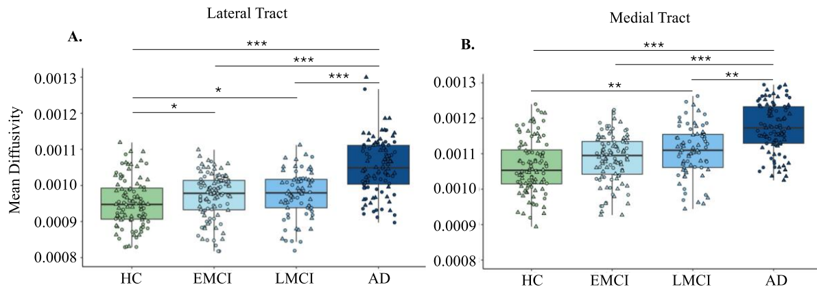
Figure 3. Comparison of the mean diffusivity of the lateral (A) and medial (B) NBM tracts across healthy controls (HC), early mild cognitive impairment (EMCI), late mild cognitive impairment (LMCI), and Alzheimer's disease (AD). Triangles: left hemisphere; Circles: right hemisphere. * p < 0.05 ; ** p < 0.01 ; *** p < 0.0001
