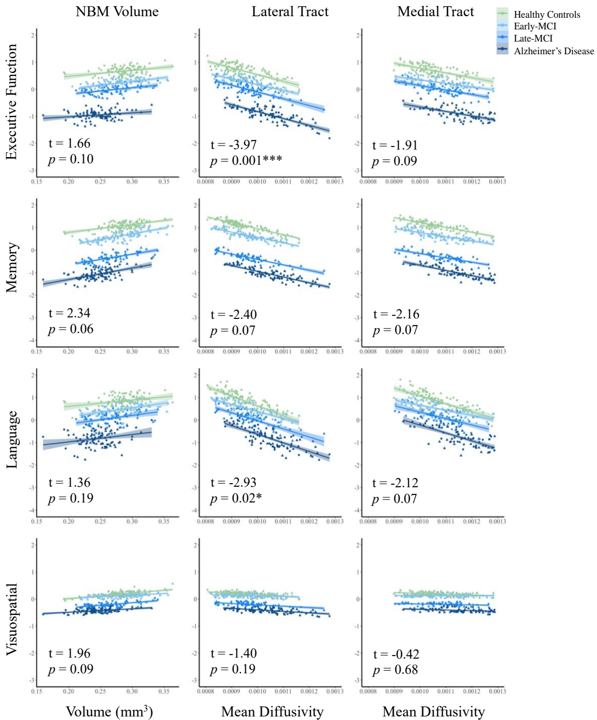
Figure 4. Predicted cognitive scores based on the linear regression models of normalized NBM volume, and mean diffusivity of both the lateral and medial NBM tracts. Triangles: left hemisphere; Circles: right hemisphere. p-values are FDR corrected. * p < 0.5 ; ** p < .001
