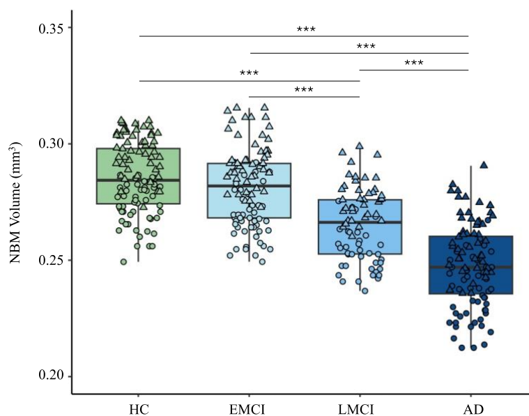
Figure 2. Comparison of NBM volume across healthy controls (HC), early mild cognitive impairment (EMCI), late mild cognitive impairment (LMCI), and Alzheimer's disease (AD). Triangles: left hemisphere; Circles: right hemisphere. *** p<0.0001
