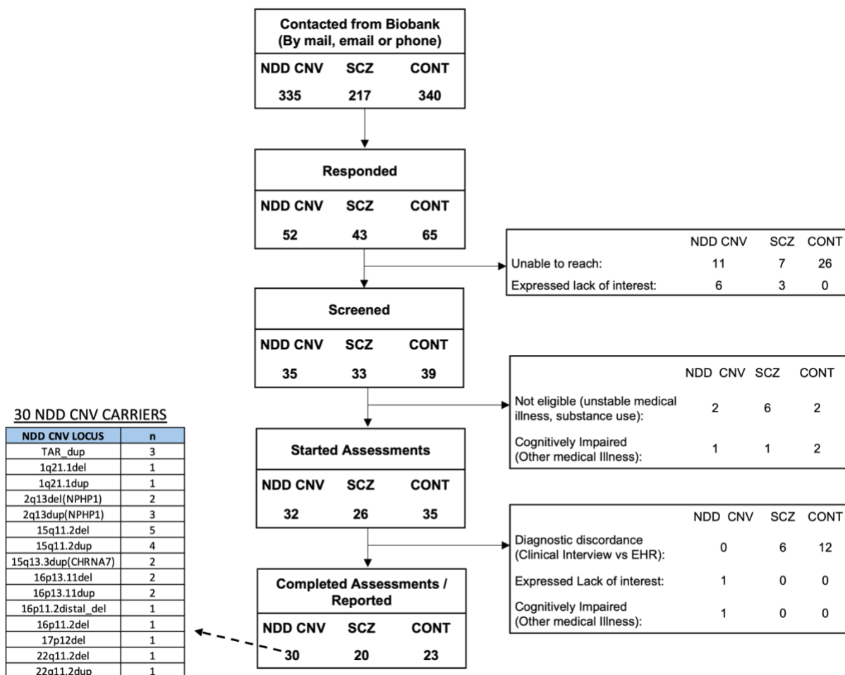
Figure 1: Study Recruitment. Flow chart of recontact of 892 biobank participants across three comparator groups, from initial stage of recontact to recruitment and study assessments. The indented table indicates the CNV loci of the 30 NDD CNV carriers who completed study assessments.
