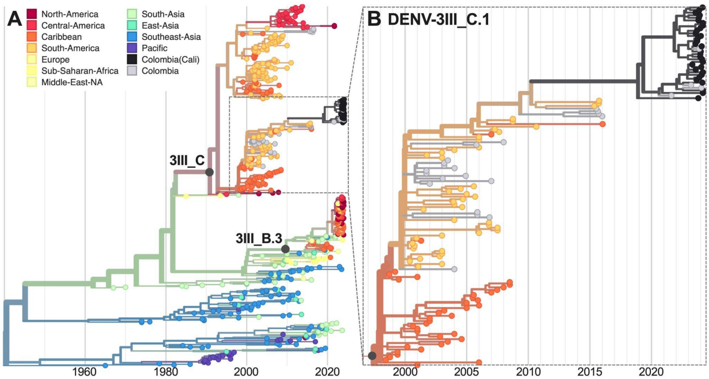
Figure 4. Time-resolved maximum-likelihood phylogeny of DENV-3. (A) Full reconstruction of 542 DENV-3 sequences colored by sampling location. (B) Zoom on the DENV-3III_C.1 clade highlighting sequences from Cali, Colombia (black).
