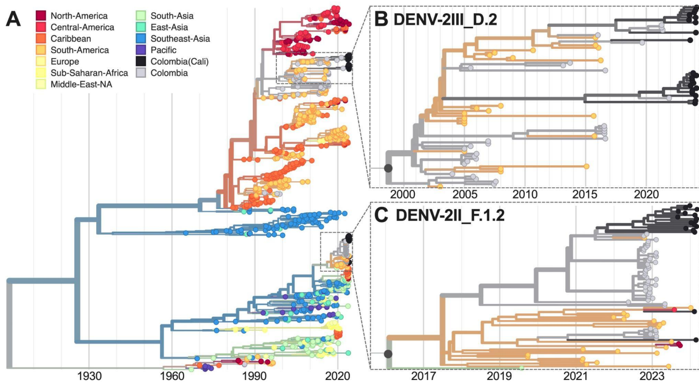
Figure 3. Time-resolved maximum-likelihood phylogeny of DENV-2. (A) Full reconstruction of 965 DENV-2 sequences colored by sampling location. Zoom on the (B) DENV-2III_D.2 and (C) DENV-2II_F.1.2 clades highlighting sequences from Cali, Colombia (black).
