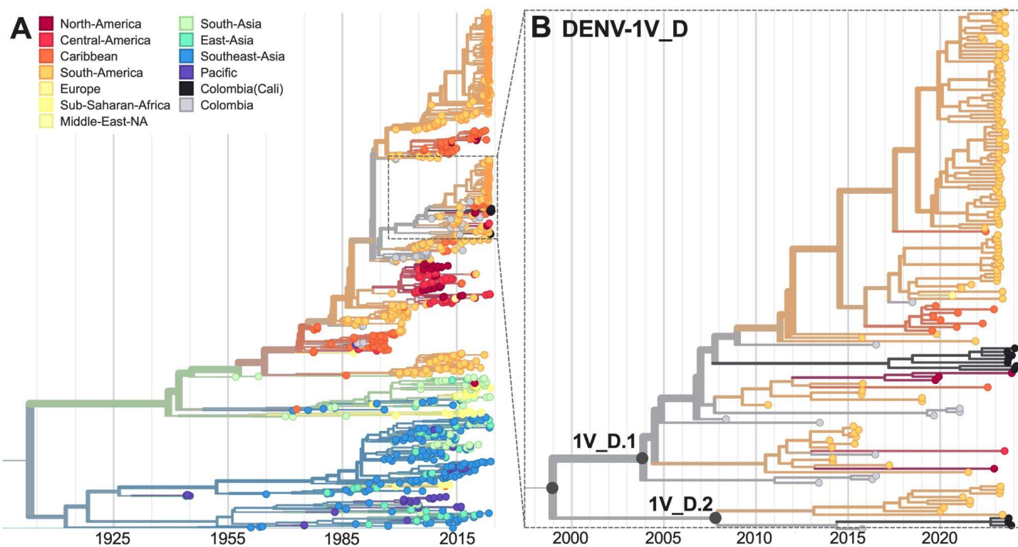
Figure 2. Time-resolved maximum-likelihood phylogeny of DENV-1. (A) Full reconstruction of 1007 DENV-1 sequences colored by sampling location. (B) Zoom on the DENV-1V_D clade highlighting sequences from Cali, Colombia (black).
