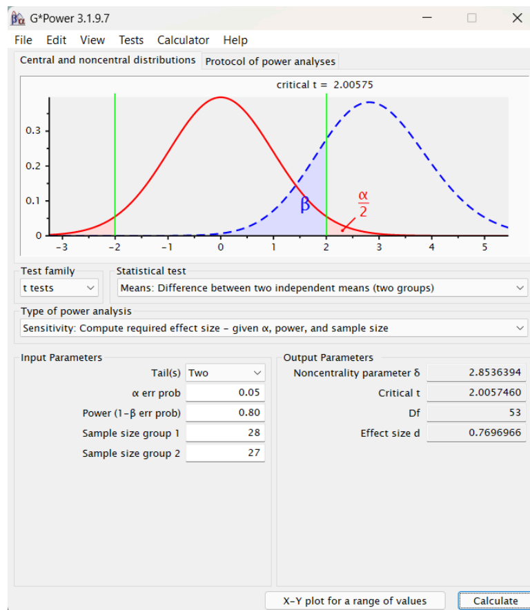
Supplementary Figure 2. Sensitivity calculation for two-sample t-test with n = 55 and power = 80%.
