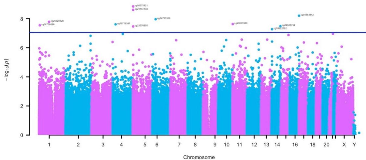
Figure 1. Manhattan Plot of the epigenome-wide association meta-analyses. The x-axis depicts chromosomes and the location of each CpG site across the genome. The y-axis depicts the -\log_{10} of the unadjusted p -value for the association with current PTSD. Each dot represents a CpG site. The solid blue line indicates the epigenome-wide statistical significance at p < 9.0e-8 .
