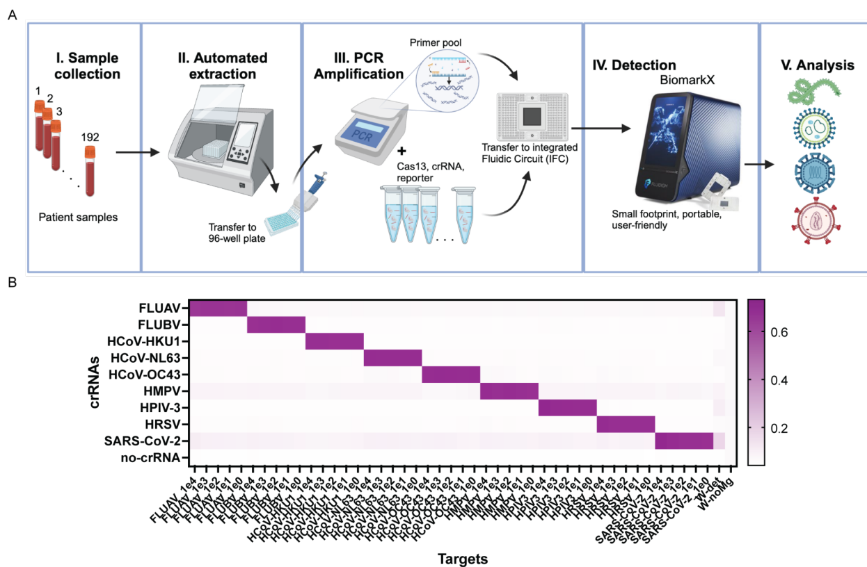
Figure 1. Robust detection of the respiratory virus panel using the CARMEN-BiomarkX. (A) Schematic of CARMEN workflow from blood samples to final results using the BiomarkX instrument from Standard BioTools. (B) Heatmaps illustrating CARMEN assay performance for the respiratory virus panel (RVP) including SARS-CoV-2, HCoV-HKU1, HCoV-OC43, HCoV-NL63, FLUAV, FLUBV, HPIV-3, HRSV, HMPV. Data shows fluorescence intensity of synthetic DNA fragments, at 10^4 - 10^0 copies per \mu\text{L} , and corresponding viral Cas13 crRNAs at 1 hour post-reaction initiation.
