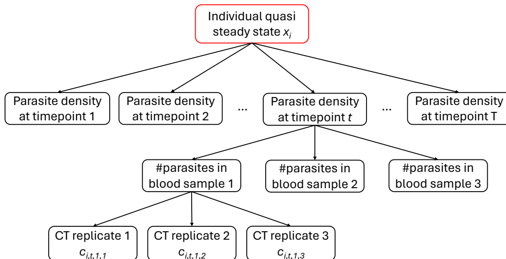
Figure 1: Graphical representation of the data structure for a given individual. We assume that individual i has a steady state trypanomastigote density in blood denoted x_i (treatment results in a step change in x_i to either 0 (cure) or a lower positive value). Stochasticity in measurement of x_i results from fluctuations over time, across blood samples, and the heteroskedastic PCR measurement error.
