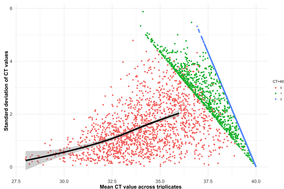
Figure S4: The relationship between the mean value and the standard deviation among all samples for which qPCR was done in triplicate and where at least one sample had a Ct value < 40 ( n=3,482 samples). The points are coloured by the number of technical replicates with a Ct value < 40. Red: all Ct values < 40; green 2/3 Ct values < 40; blue: 1/3 Ct values < 40. The black line shows a spline fit to the data with all three triplicates < 40 (red points) with mean value between 27 and 36 (above 36 the spline fit is biased downwards).
