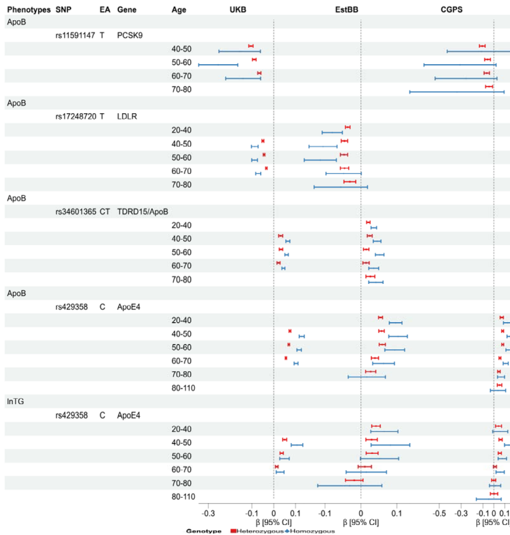
Figure 2. Associations between the genotypes of the lead SNPs and the corresponding phenotypes for age-stratified analyses in UKB and two validation cohorts. ApoB, apolipoprotein B; EA, effect allele; SNP: single nucleotide polymorphism; TG: triglyceride. Cohort names: UKB, UK Biobank; EstBB, Estonian Biobank; CGPS, Copenhagen General Population Study. In UKB and EstBB, linear regressions were adjusted for sex and the first ten genetic principal components, whereas in CGPS only sex was adjusted. For EstBB, the figure showed the results of rs62122481 (effect allele: A), which is a proxy SNP for rs34601365.
