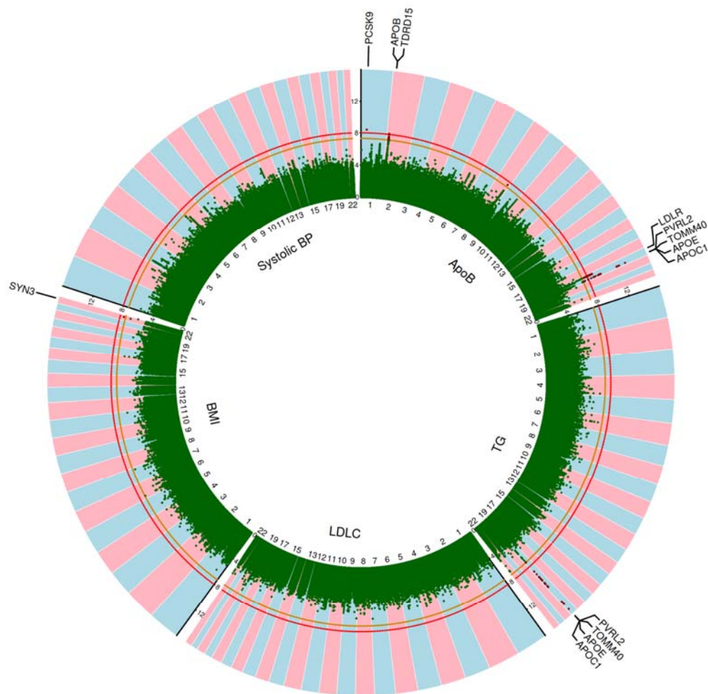
Figure 1. Circular Manhattan plot for the log-transformed (base 10) P -values of the interaction terms between genetic variants and age. Abbreviations in clockwise direction: ApoB, apolipoprotein B; TG, triglyceride; LDLC, low-density lipoprotein cholesterol; BMI, body mass index; BP, blood pressure. The orange line indicates a P -value of 5e-8, and the red line indicates a P -value of 1e-8 after Bonferroni correction for multiple testing. Red dots indicate genome-wide significant SNPs with P -values smaller than 5e-8 for the interaction terms. Labelled gene names in black were identified by FUMA.
