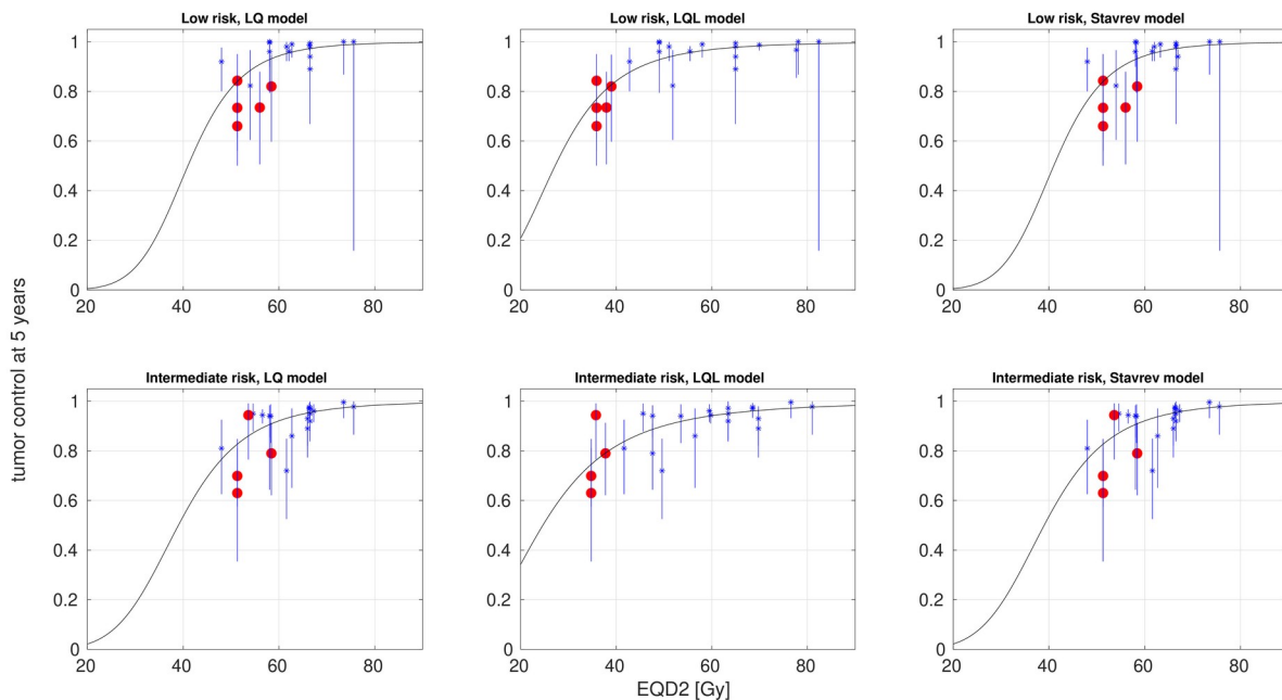
Figure 2: Best fits of LQ, LQL, and Stavrev's reoxygenation models to dose–response data for prostate cancer treated with HDR-BT (low risk, top panels; intermediate risk, bottom panels). The \alpha/\beta ratio was constrained to be low ( 1 \leq \alpha/\beta \leq 8 Gy). Clinical data (*) and 95% confidence intervals (bars), and modeled curves (solid lines). Single fraction schedules are highlighted as red circles.
