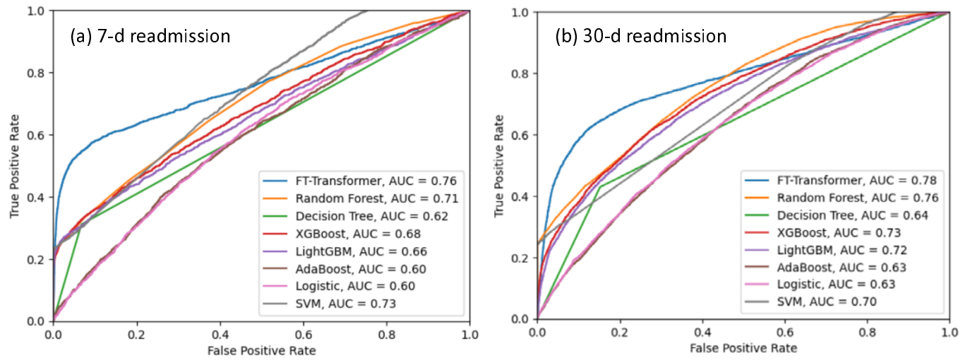
Figure 1 ROC Curves for Different ML Algorithms. This figure compares the performance of various machine learning algorithms in predicting (a) 7-day readmission and (b) 30-day readmission.
