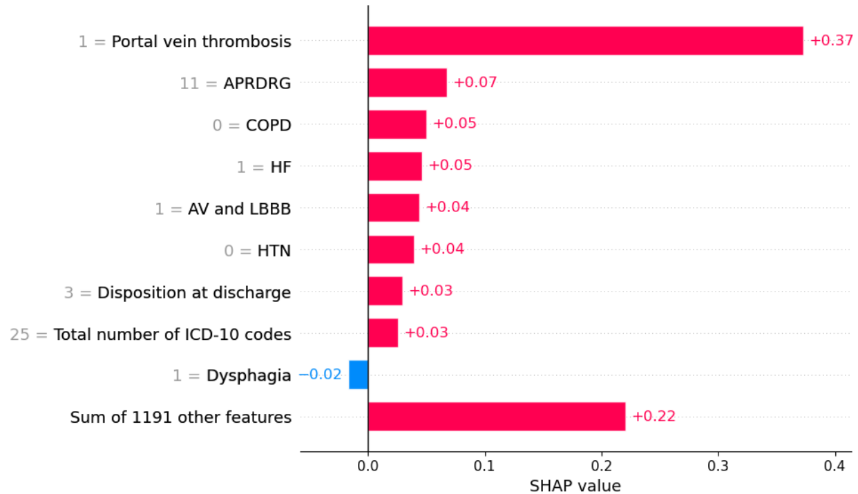
Figure 4 Feature Contributions for Predicting 7-Day Readmission. This figure displays the feature contributions for a specific individual who was readmitted within 7 days. The model predicted the readmission with a high probability of 0.99.
