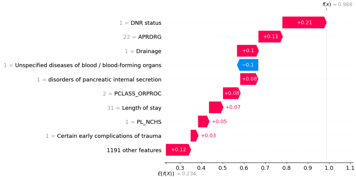
Figure A. 1 Feature Contributions for Predicting 30-Day Readmission. This figure displays the feature contributions for a specific individual who was readmitted within 30 days. The model predicted the readmission with a high probability of 0.988.
