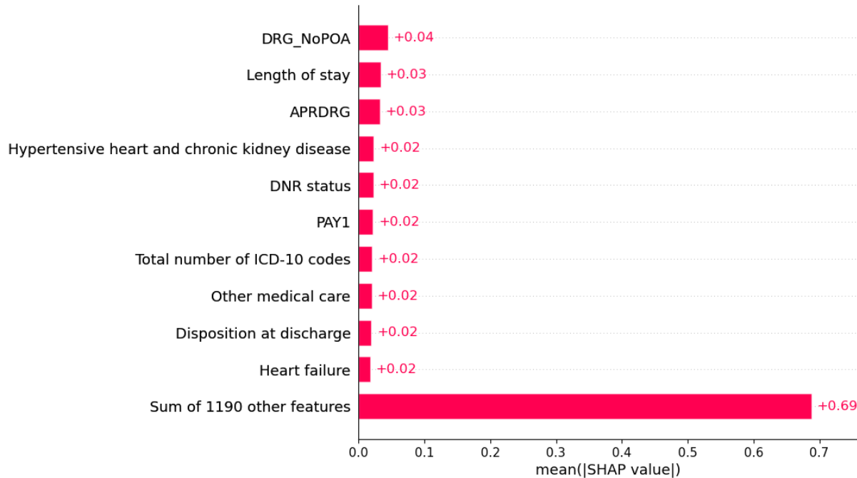
Figure 3 Feature Contributions to Predicting 30-Day Readmission.
