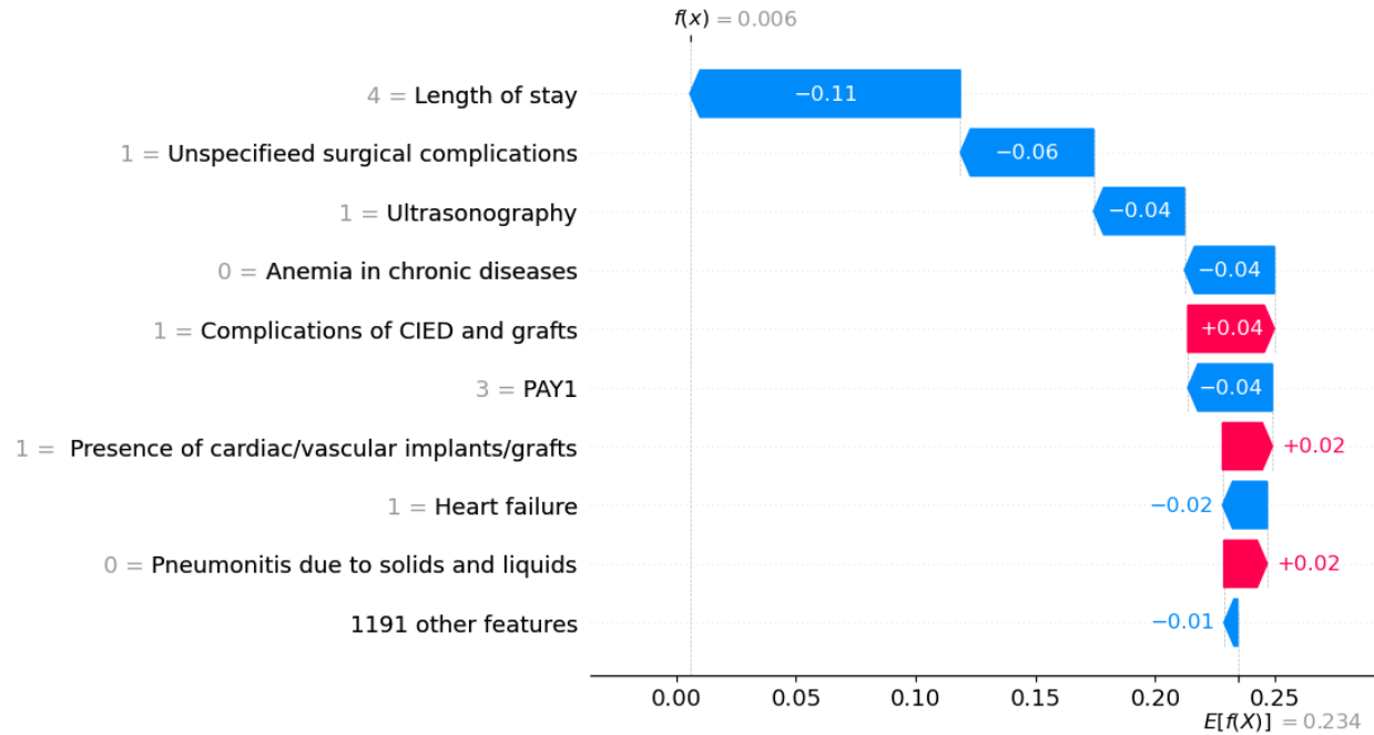
Figure A. 2 Feature Contributions for Predicting 30-Day Readmission. This figure illustrates the feature contributions for a specific individual who was not readmitted within 30 days. The model predicted a low readmission probability of 0.006, effectively indicating a negligible likelihood of readmission.
