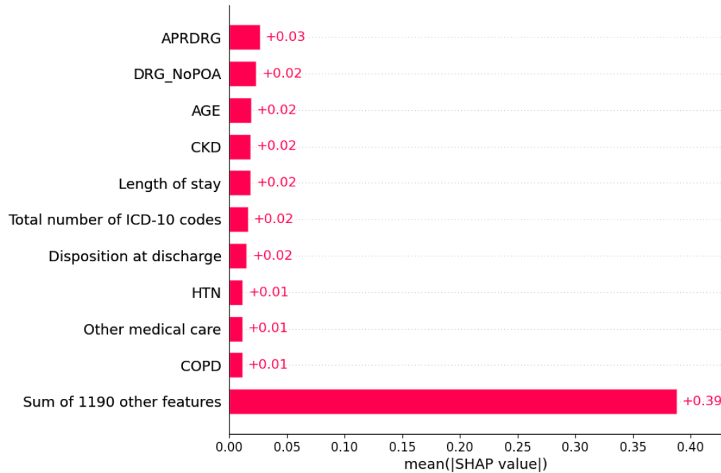
Figure 2 Feature contributions to predicting 7-day readmission in study population. APRDRG: All patient refined diagnosis related groups, which is an index of case severity and complexity used for insurance reimbursement; DRG_NoPOA: Diagnosis related groups assignment made without the use of the present on admission flags for the diagnoses; CKD: Chronic kidney disease; HTN: Essential hypertension; Other medical care: including palliative care, blood transfusion, chemotherapy or radiation therapy for neoplasm or other unspecified medical care; COPD: chronic obstructive pulmonary disease and heart failure.
