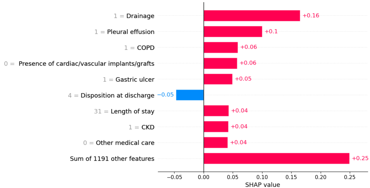
Figure 5 Feature Contributions for Predicting 30-Day Readmission. This figure displays the feature contributions for a specific individual who was readmitted within 30 days. The model predicted the readmission with a high probability of 0.99.
