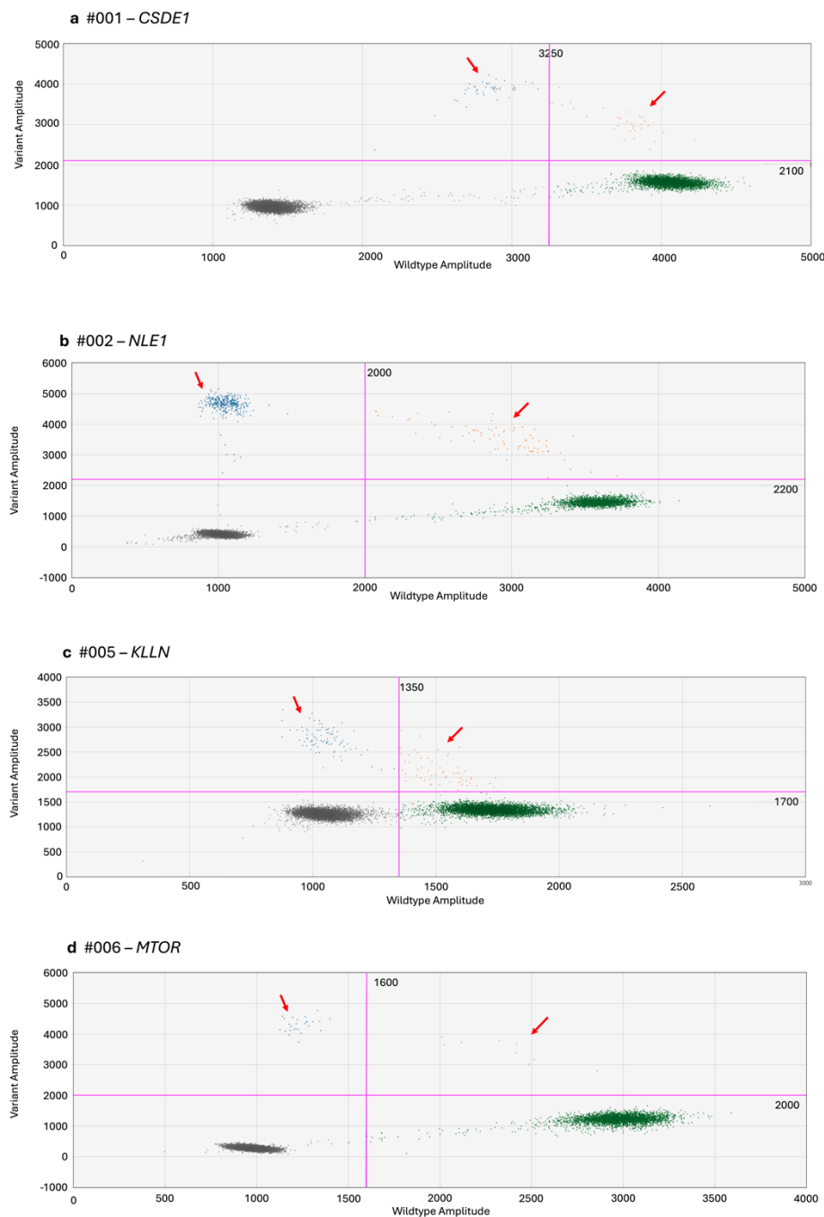
Fig. 3: ddPCR results for candidate variants in affected brain regions showing variant confirmation in affected samples (a-d). Due to technical issues (GC-rich region), the KLLN assay did separate less well between positive and negative variant droplets. Gating was determined based on fluorescent intensities of no template control samples. Blue: variant droplets, green: wild-type droplets, orange: droplets containing multiple DNA templates, gray: empty droplets, red arrows are showing bulk of variant droplets for CSDE1 , NLE1 , KLLN and MTOR . ddPCR results for candidate variants in unaffected brain regions and germline samples are available as Extended Data Fig. 1.
